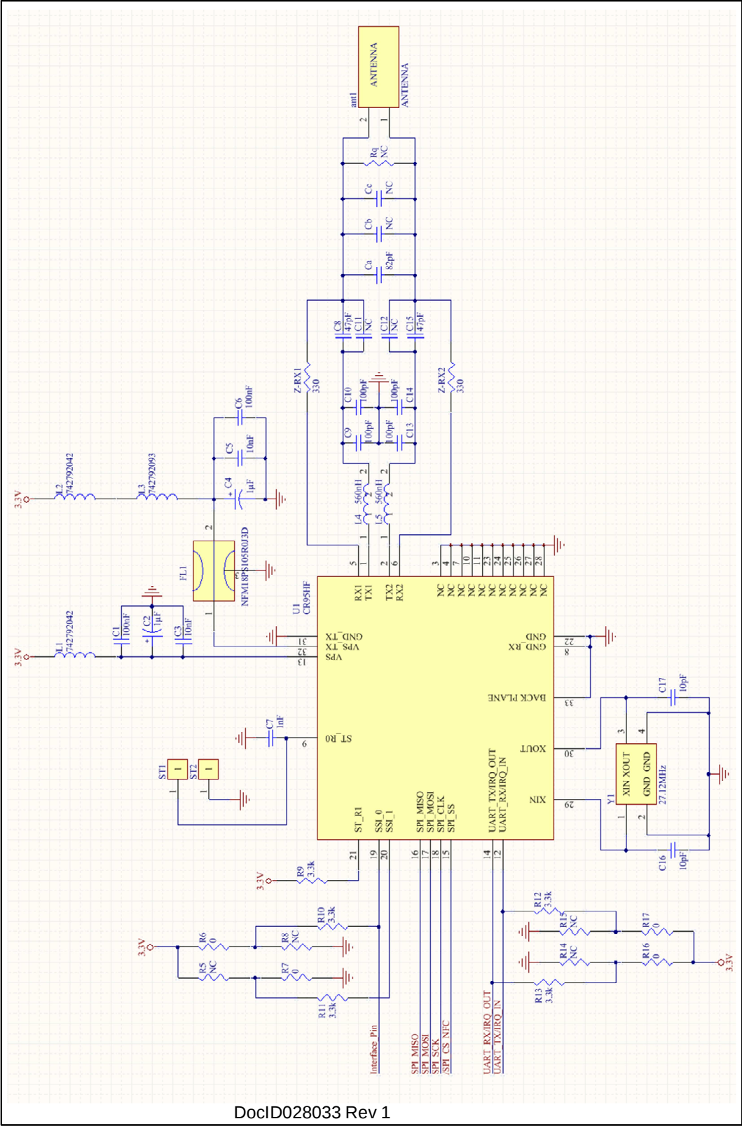
Figure 5: CR95HF
