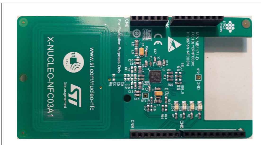
Figure 1: NFC card reader board based on CR95HF IC
