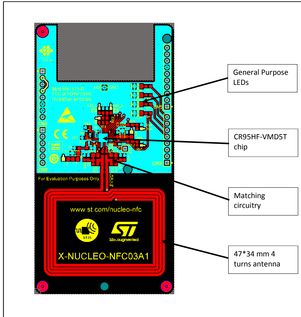
Figure 3: X-NUCLEO-NFC03A1 component placement details
