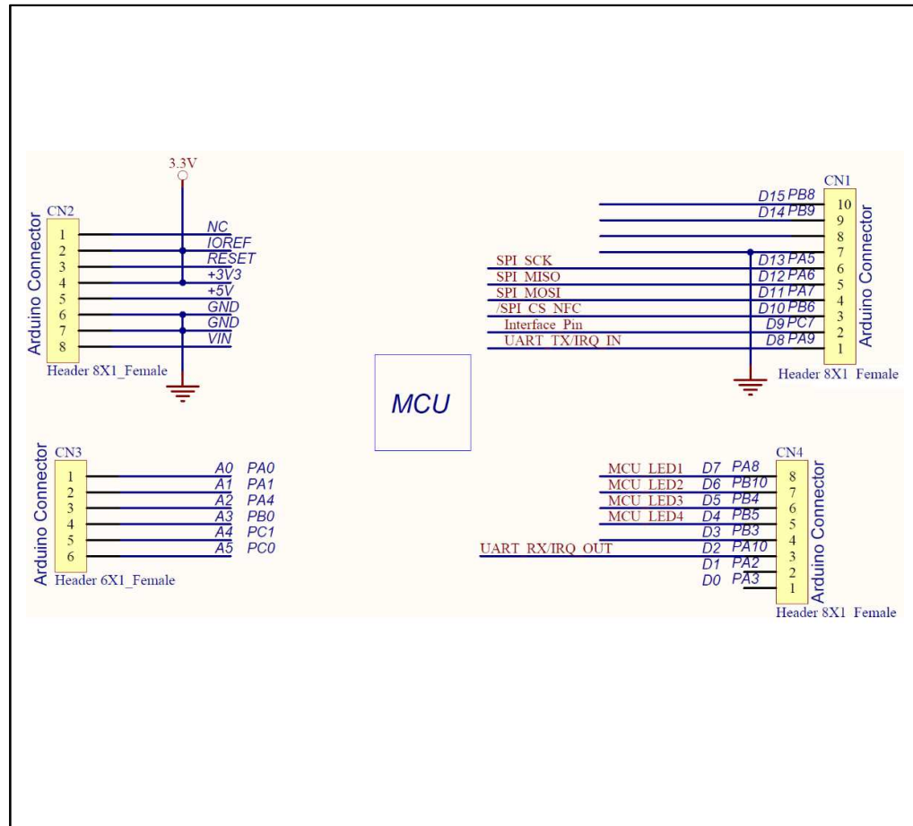
Figure 4: Nucleo connectors
