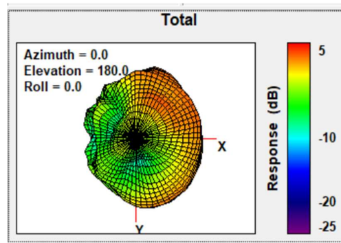
Total Gain Bottom view 2402MHz
