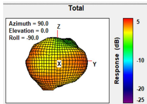
Total Gain Left Side view 2402MHz
