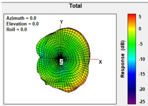
Total Gain Top view 2440MHz
