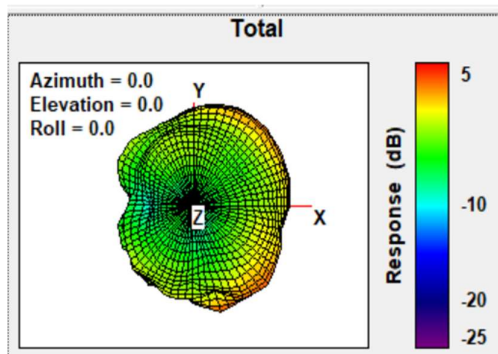
Total Gain Top view 2402MHz
