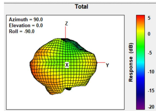
Total Gain Left Side view 2480MHz
