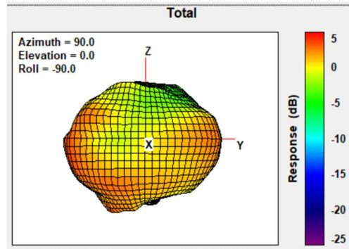
Total Gain Left Side view 2440MHz
