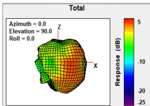
Total Gain Back Face view 2402MHz
