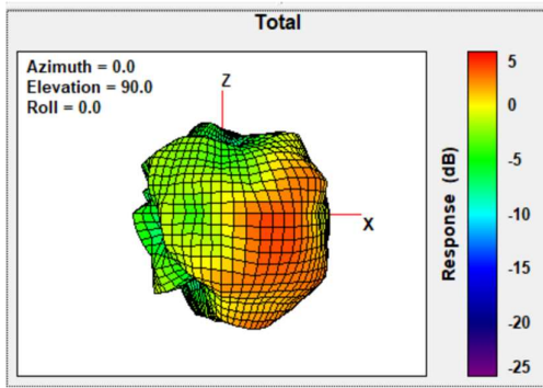
Total Gain Back Face view 2440MHz
