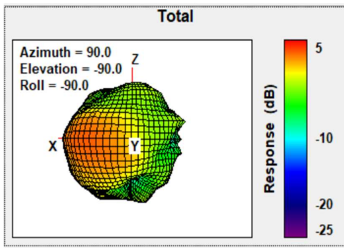
Total Gain Front Face view 2402MHz
