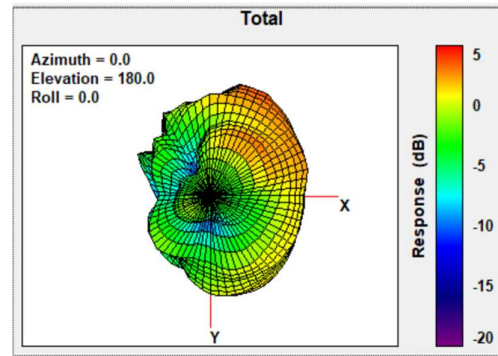
Total Gain Bottom view 2480MHz
