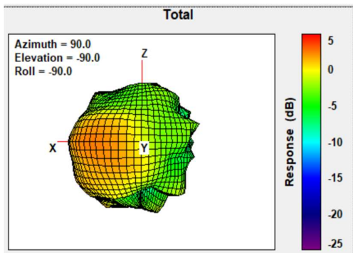
Total Gain Front Face view 2440MHz
