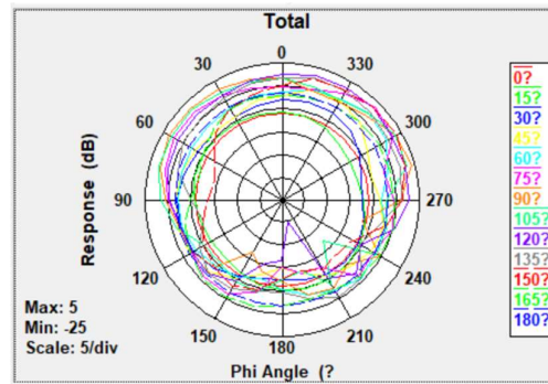
Total Gain Right Side view 2402MHz
