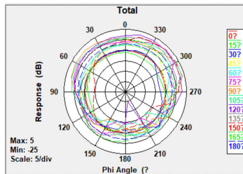
Total Gain Right Side view 2440MHz
