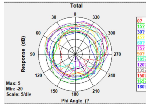
Total Gain Right Side view 2480MHz
