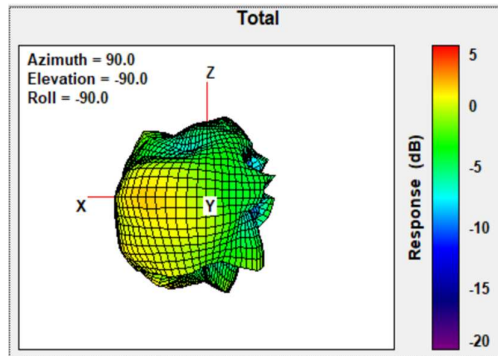
Total Gain Front Face view 2480MHz
