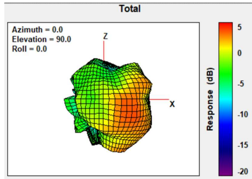
Total Gain Back Face view 2480MHz
