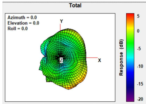
Total Gain Top view 2480MHz
