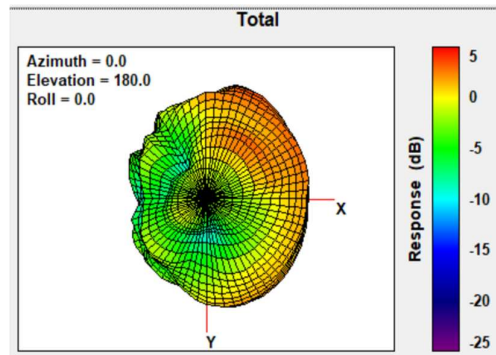
Total Gain Bottom view 2440MHz
