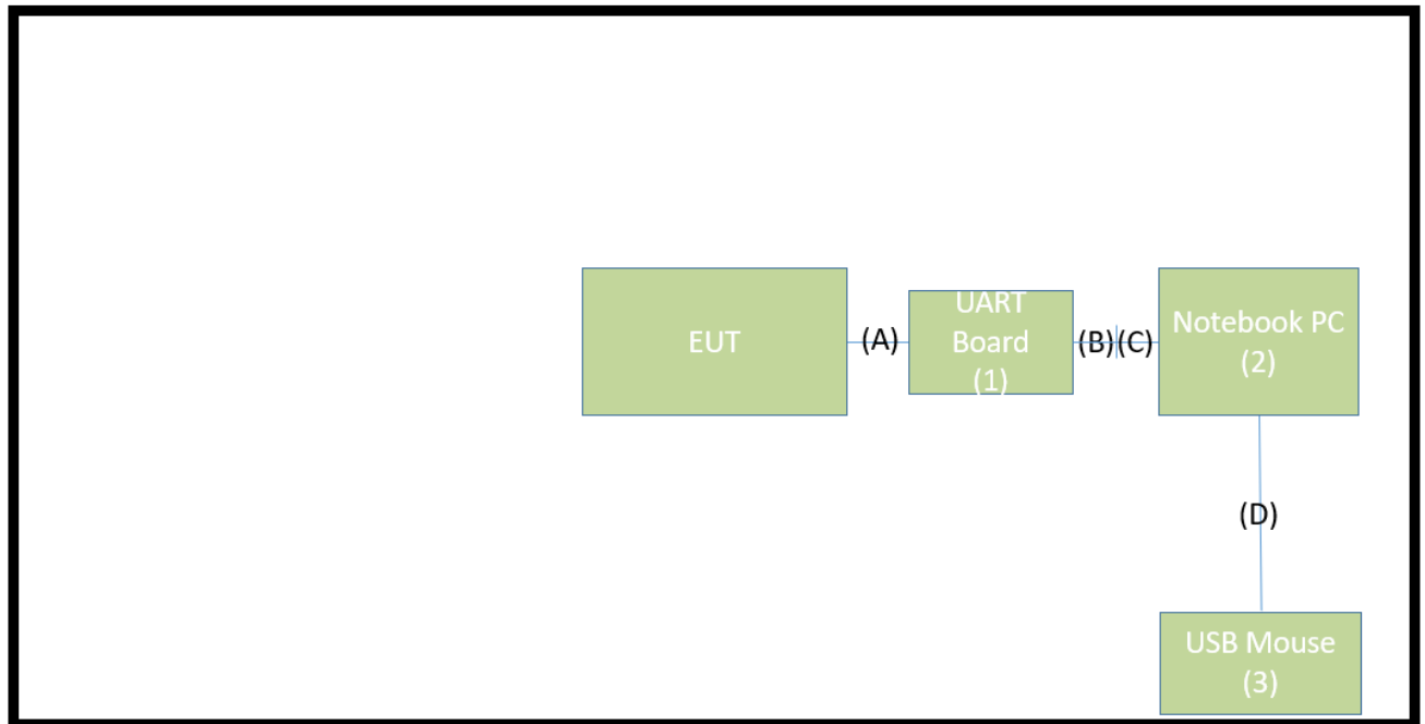
Connection Diagram – Mode1~8
