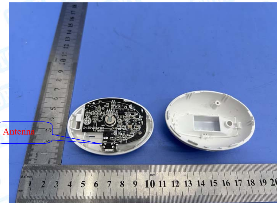
Photo 6 Internal of EUT
