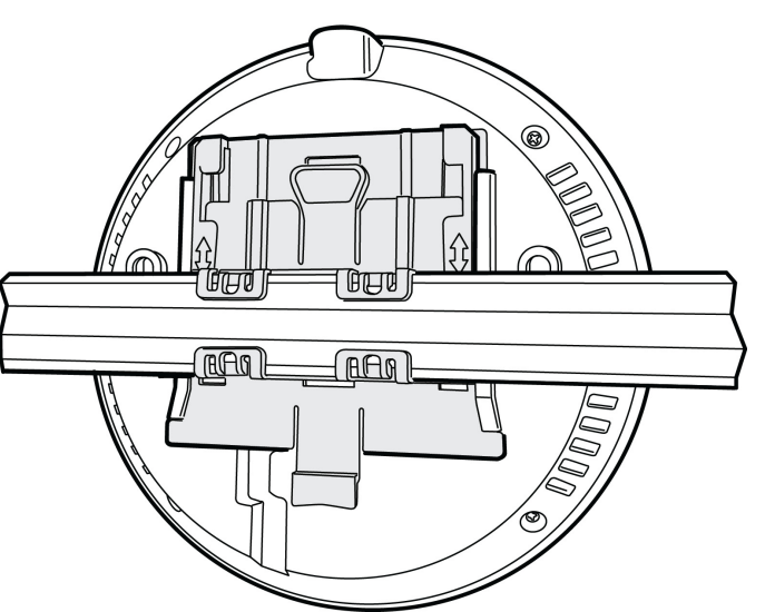
Figure 3 Mounting Bracket on T-bar
