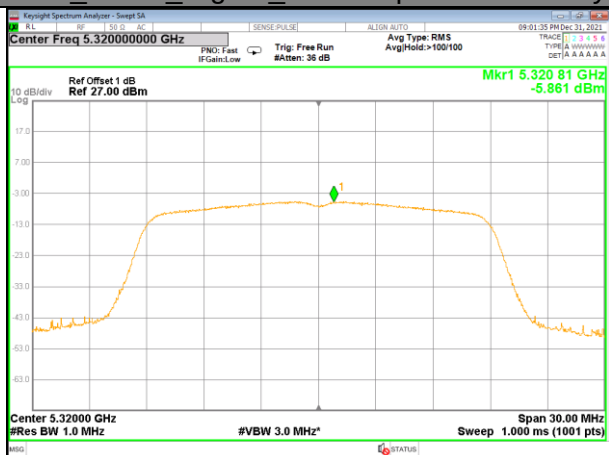
W53_11n20_Higher_Power Spectrum Density
