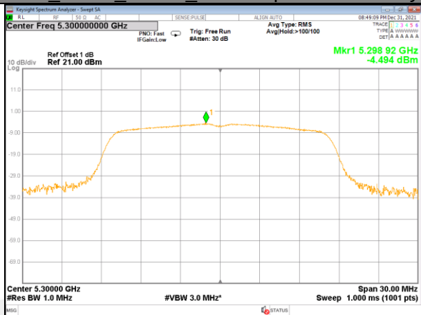
W53_11n20_Lower_Power Spectrum Density
