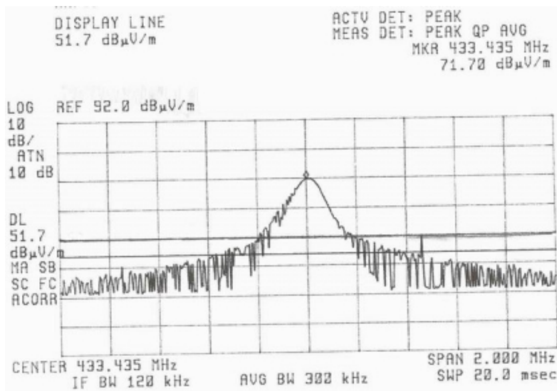
Figure 6.2 Occupied Bandwidth
