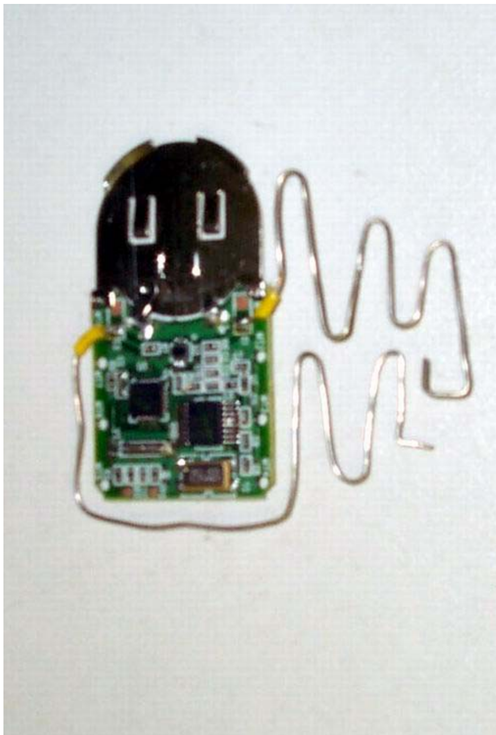
PCB Component View
