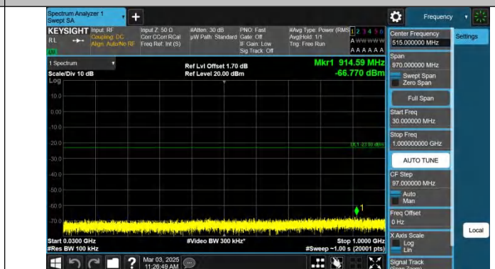
Band4-3MHz-QPSK-19965-1RB#14-30~1000-PASS
