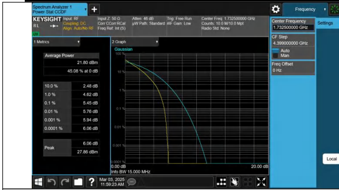
Band4-15MHz-QPSK-20175-75RB#0-PASS
