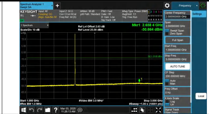
Band4-3MHz-QPSK-19965-1RB#0-1000~3000-PASS
