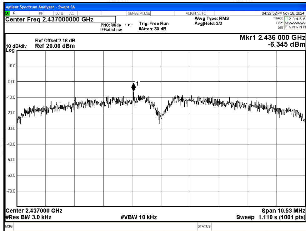
PSD NVNT b 2437MHz Ant6
