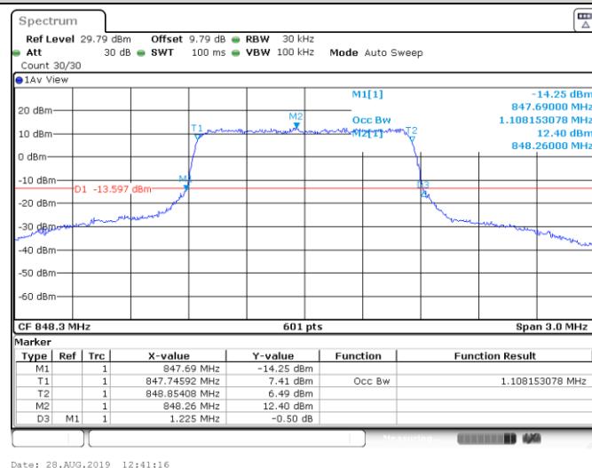
Band5-1.4MHz-QPSK-20643-6RB#0-1.108
