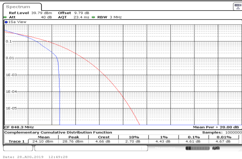
Band5-1.4MHz-QPSK-20643-6RB#0
