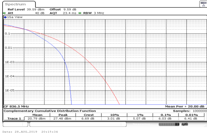
Band5-3MHz-16QAM-20635-1RB#0
