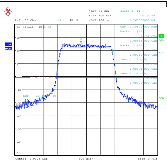
Band2-1.4MHz-16QAM-19193-6RB#0-PASS
