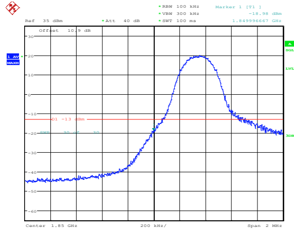
Band2-5MHz-16QAM-18625-1RB#24
