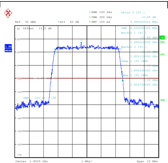
Band2-5MHz-16QAM-18625-25RB#0-PASS
