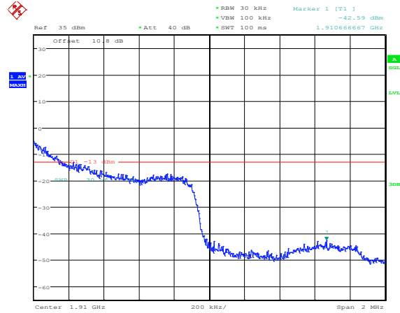
Band2-1.4MHz-16QAM-19193-1RB#5
