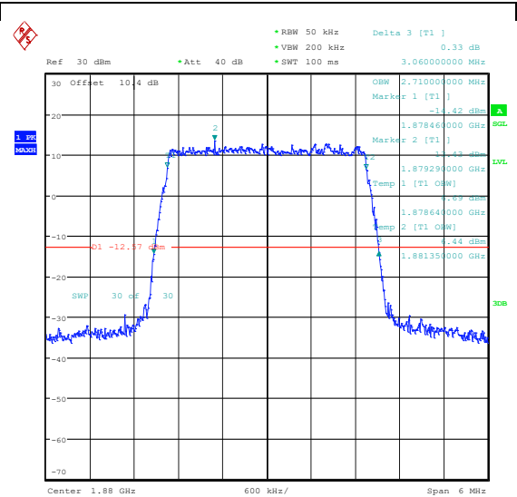
Band2-3MHz-16QAM-18900-15RB#0-PASS
