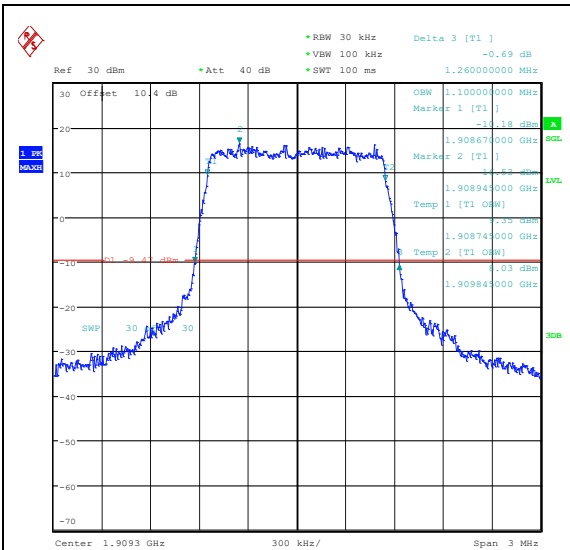
Band2-1.4MHz-QPSK-19193-6RB#0-PASS
