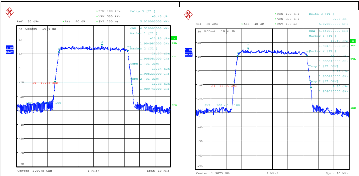
Band2-5MHz-QPSK-19175-25RB#0-PASS Band2-5MHz-16QAM-19175-25RB#0-PASS
