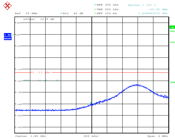
Band2-10MHz-16QAM-18650-1RB#49
