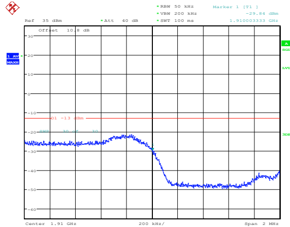
Band2-3MHz-16QAM-19185-1RB#14
