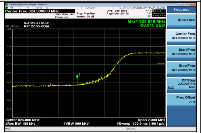
LCH_16QAM_50RB#0
