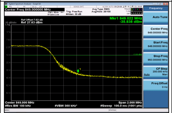
HCH_16QAM_50RB#0
