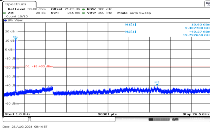
11B_Ant1_2437_1000-26500
