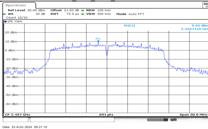
11G_Ant1_2437_0~Reference
