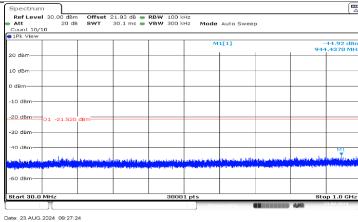
11N20SISO_Ant1_2437_30~1000
