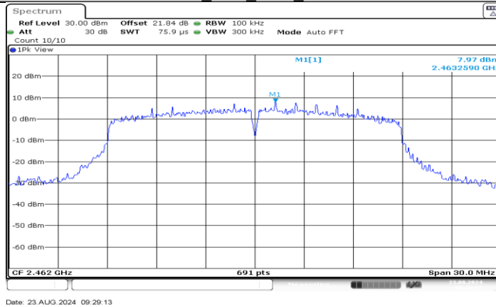
11N20SISO_Ant1_2462_0~Reference
