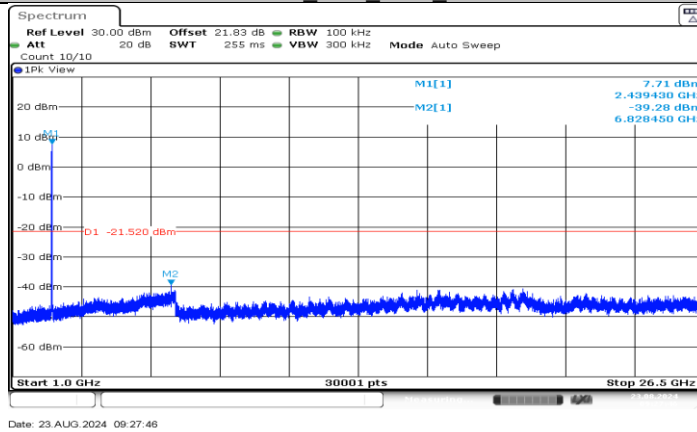
11N20SISO_Ant1_2437_1000~26500
