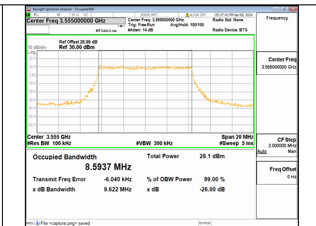
n48 10M DFT-s-OFDM QPSK Outer_Full Low
