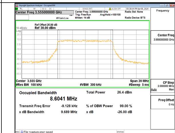
n48 10M DFT-s-OFDM 64QAM Outer_Full Low
