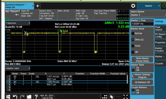
802.11ac-VHT40(T=5.390ms)
