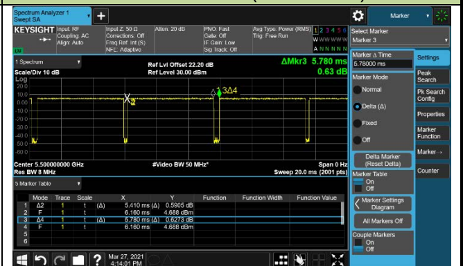
802.11ac-VHT80(T=5.400ms)
