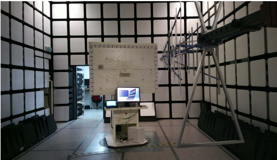
Picture 2. FCC Part 15B Radiated emissions
