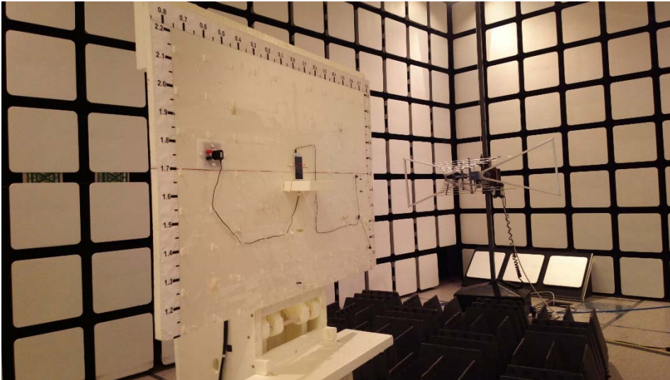
Picture 1. FCC Part 15C Radiated emissions
