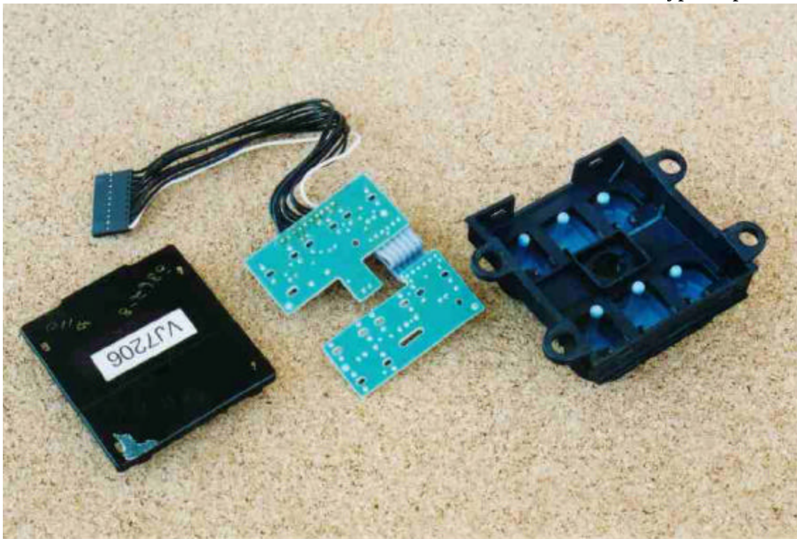
CPSIHL3 Keypad Open - Top
