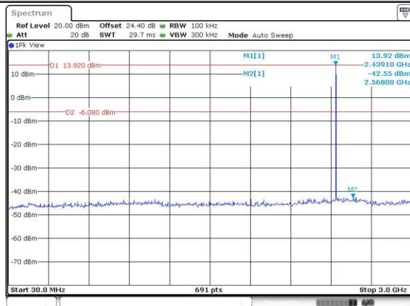
CSE Plot on CH 39 between 30 MHz ~ 3 GHz
