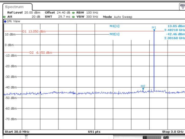
CSE Plot on CH 78 between 30 MHz ~ 3 GHz
