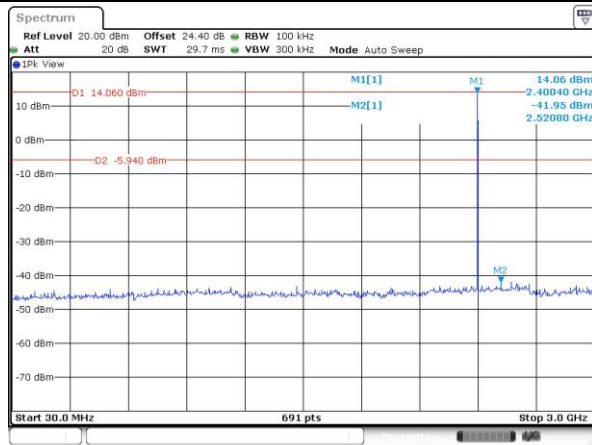
CSE Plot on CH 00 between 30 MHz ~ 3 GHz
