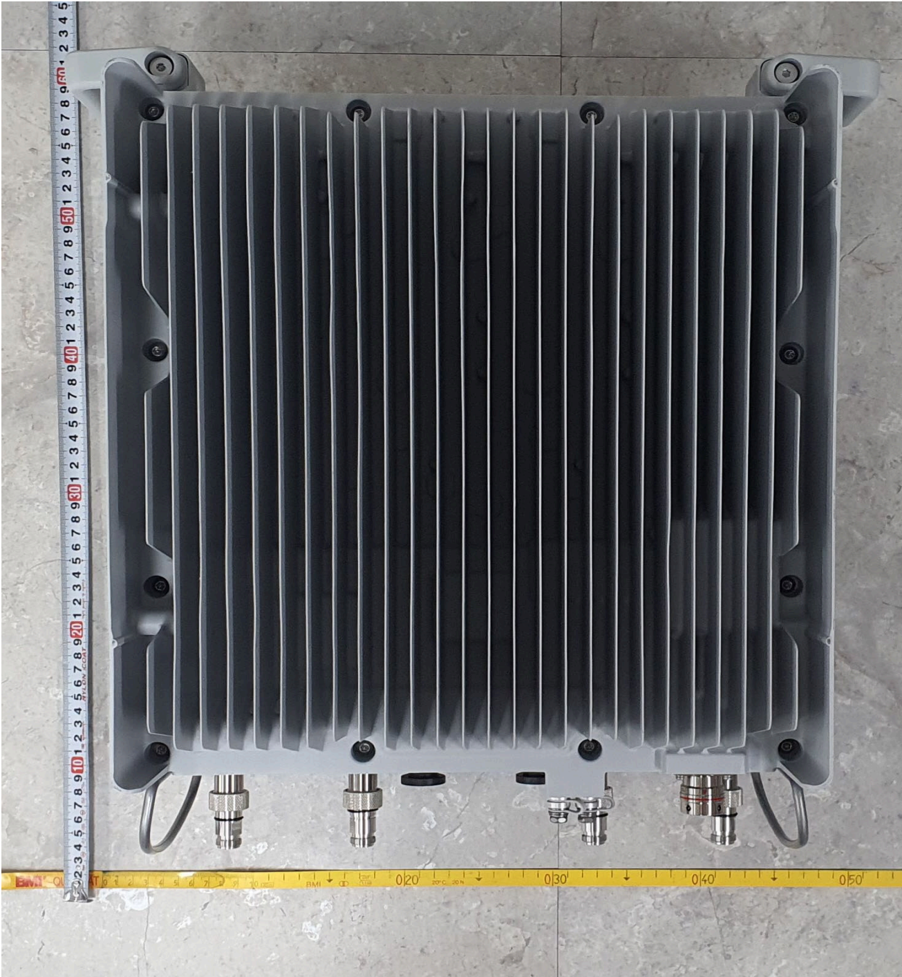
Front view
