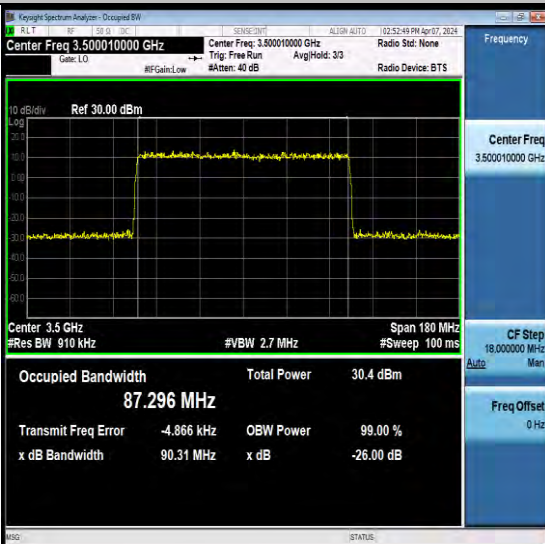
NTNV-N78-3450-3550-PC2-30-90-M-CP-64QAM-Outet_Full-A Ant3-PASS
