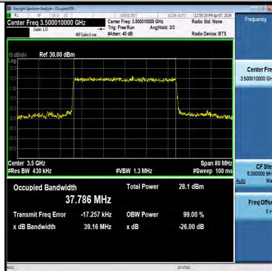
NTNV-N78-3450-3550-PC2-30-40-M-CP-256QAM-Outer_Full-Ant5-PASS
