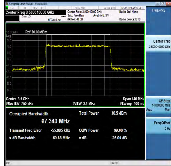
NTNV-N78-3450-3550-PC2-30-70-M-CP-256QAM-Outet_Full-A nt3-PASS
