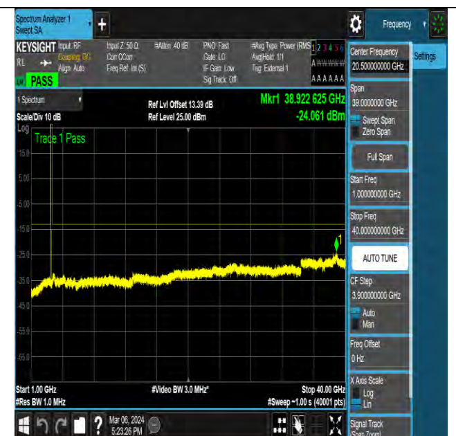
NTNV-N78-3450-3550-PC2-30-20-L-DFT-QPSK-Edge_1RB_ Left-Ant5-PASS
