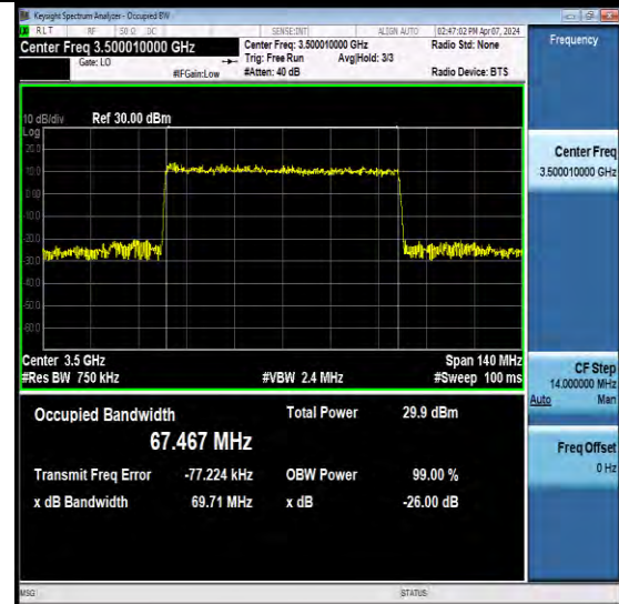
NTNV-N78-3450-3550-PC2-30-70-M-CP-256QAM-Outer_Full-Ant5-PASS
