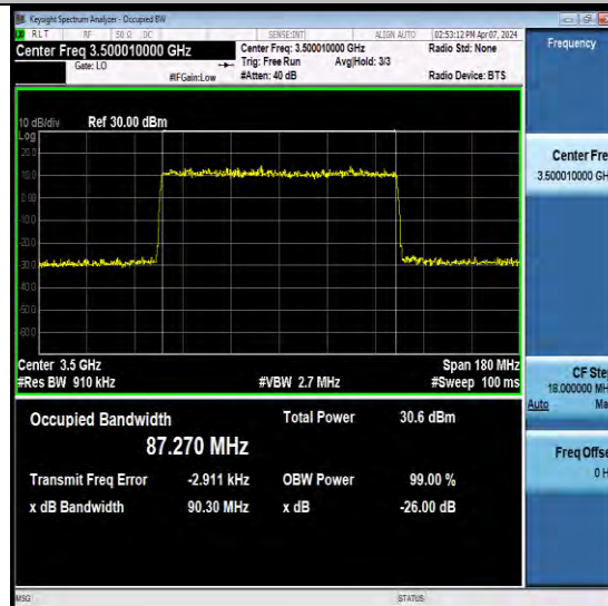
NTNV-N78-3450-3550-PC2-30-90-M-CP-256QAM-Outet_Full-A I-Ant3-PASS
