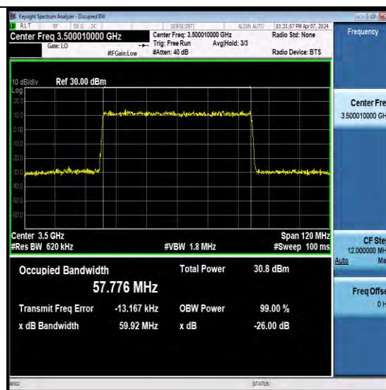
NTNV-N78-3450-3550-PC2-30-60-M-CP-16QAM-Outer_Full-Ant3-PASS
