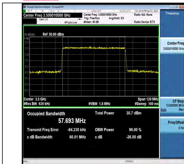
NTNV-N78-3450-3550-PC2-30-60-M-CP-QPSK-Outer_Full-Ant3-PASS
