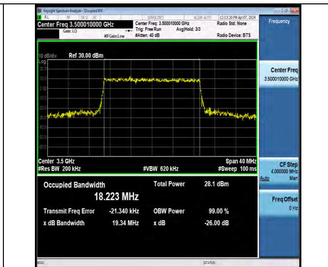
NTNV-N78-3450-3550-PC2-30-20-M-CP-16QAM-Outer_Full-Ant5-PASS
