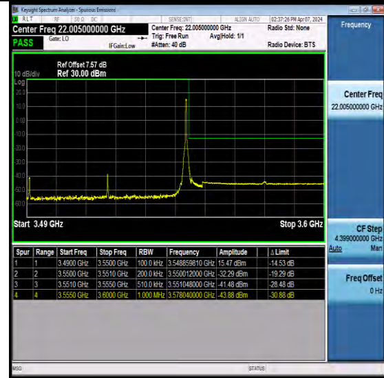
NTNV-N78-3450-3550-PC2-30-60-H-CP-QPSK-Edge_1RB_ Right-Ant3-PASS
