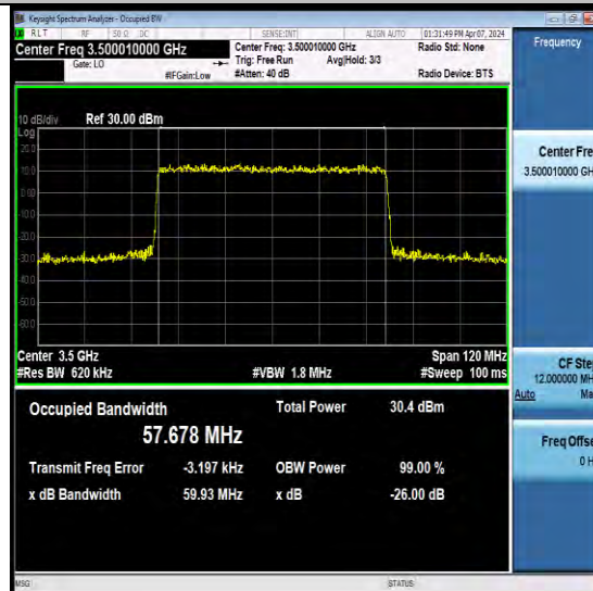
NTNV-N78-3450-3550-PC2-30-60-M-CP-256QAM-Outer_Full-Ant3-PASS
