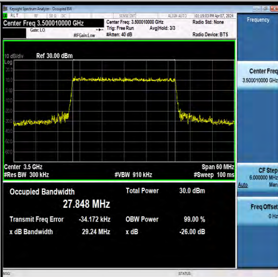
NTNV-N78-3450-3550-PC2-30-30-M-CP-64QAM-Outer_Full-Ant5-PASS
