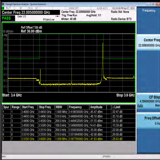
NTNV-N78-3450-3550-PC2-30-100-M-CP-QPSK-Edge_1RB Right-Ant5-PASS
