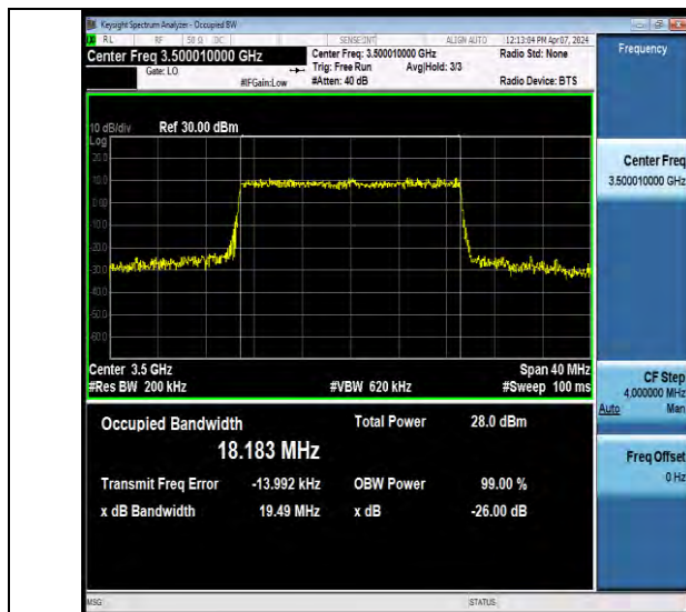
NTNV-N78-3450-3550-PC2-30-20-M-CP-QPSK-Outer_Full-Ant5-PASS
