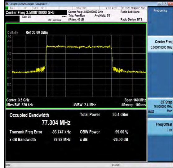
NTNV-N78-3450-3550-PC2-30-80-M-CP-256QAM-Outet_Full-A I-Ant3-PASS
