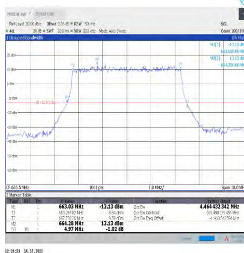
1-N71-15-5-L-2-DFT-PI2BPSK-Outer_Full-25@0-Ant1-4 1-4.464-4.970-≤5-PASS
