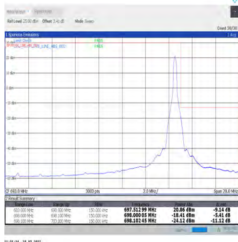
1-N71-15-15-H-2-DFT-PI2BPSK-Edge_1RB_Right-1@78-Ant1-PASS-see graph
