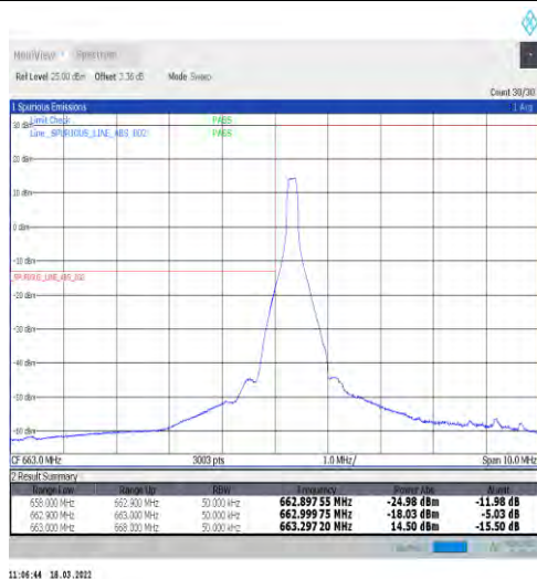
1-N71-15-5-L-4-CP-QPSK-Edge_1RB_Left-1@0-Ant1-PASS-see graph
