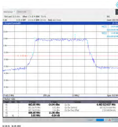
1-N71-15-5-L-4-DFT-64QAM-Outer_Full-25@0-Ant1-4 4.484-5.050-≤5-PASS
