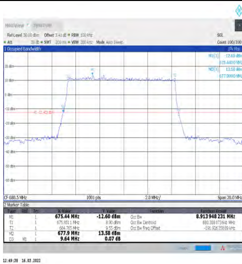
1-N71-15-10-M-1-DFT-QPSK-Outer_Full-50@0-Ant1 -8.914-9.640≤10-PASS
