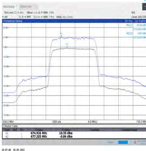
1-N71-15-20-M-1-DFT-256QAM-Outer_Full-100@0-A Ant1-11.19-100%-0.00-11.19-PASS-≤13
