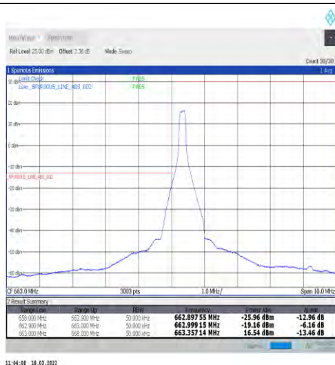
1-N71-15-5-L-1-DFT-PI2BPSK-Edge_1RB_Left-1@0-Ant1-PASS-see graph
