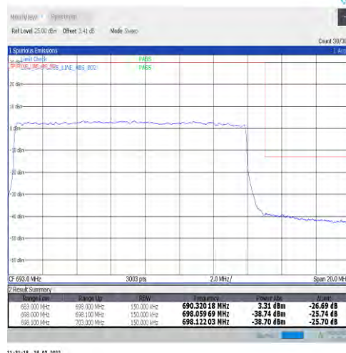
1-N71-15-15-H-3-DFT-PI2BPSK-Outer_Full-75@0-Ant1-PASS-see graph
