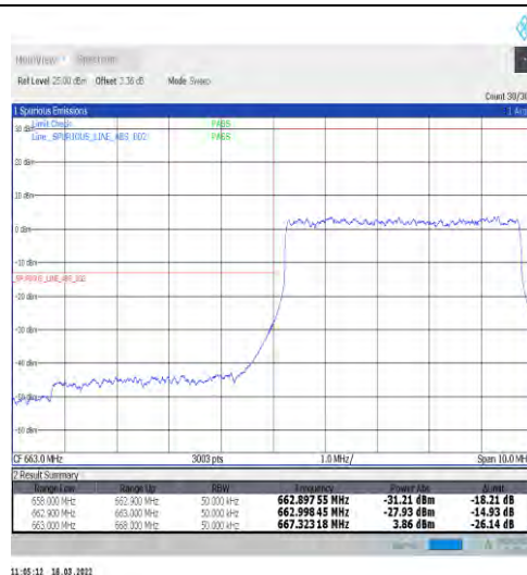
1-N71-15-5-L-3-DFT-PI2BPSK-Outer_Full-25@0-Ant1-PASS-see graph
