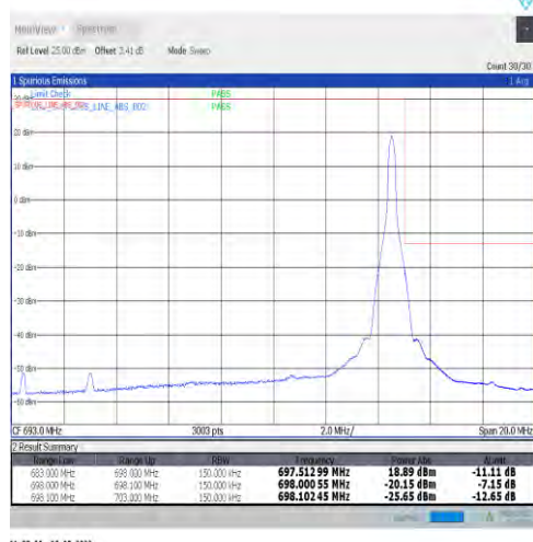
1-N71-15-15-H-5-CP-QPSK-Edge_1RB_Right-1@78-Ant1-PASS-see graph
