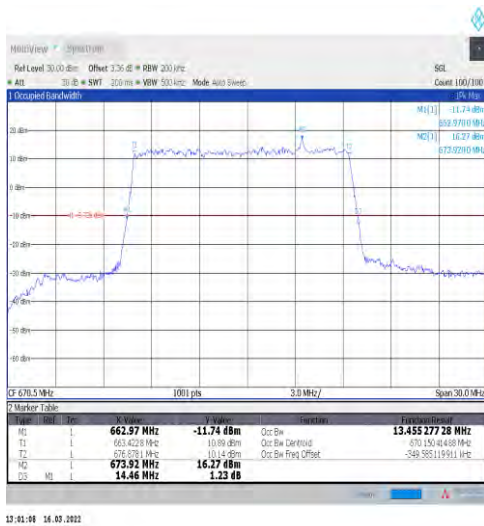
1-N71-15-15-L-1-DFT-QPSK-Outer_Full-75@0-Ant1- 13.455-14.460≤15-PASS
