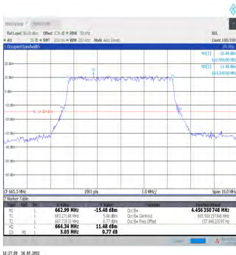
1-N71-15-5-L-3-DFT-16QAM-Outer_Full-25@0-Ant1-4 -4.456-5.050-≤5-PASS
