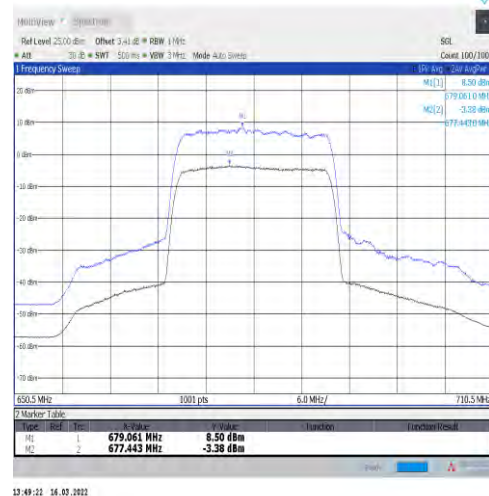
1-N71-15-20-M-2-CP-256QAM-Outer_Full-106@0-A nt1-11.88-100%-0.00-11.88-PASS-≤13
