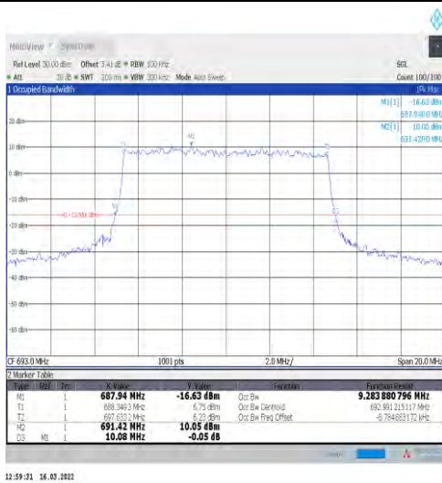
1-N71-15-10-H-8-CP-64QAM-Outer_Full-52@0-Ant1 -9.284-10.080≤10-PASS
