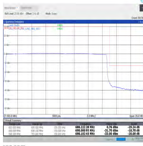
1-N71-15-15-H-6-CP-QPSK-Outer_Full-79@0-Ant1-PASS-see graph
