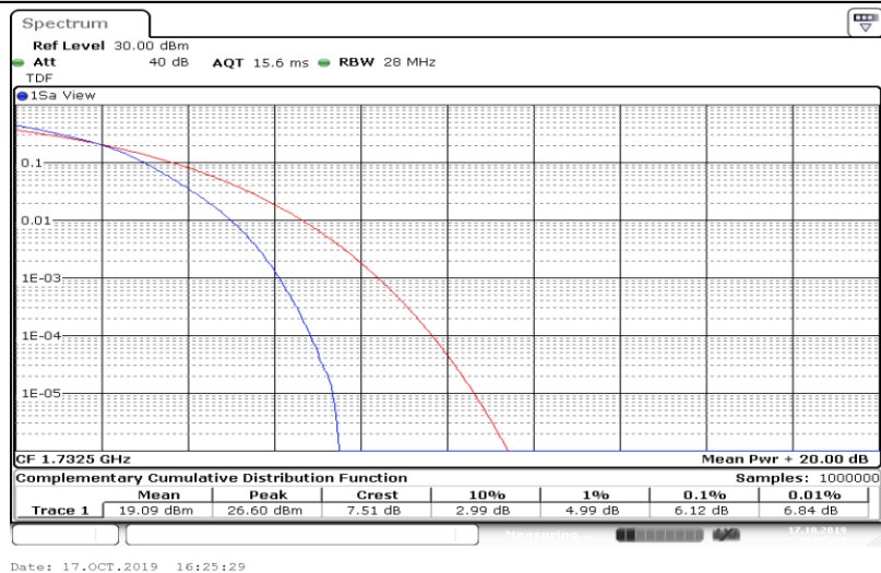
Band4-20MHz-16QAM-20300-100RB#0
