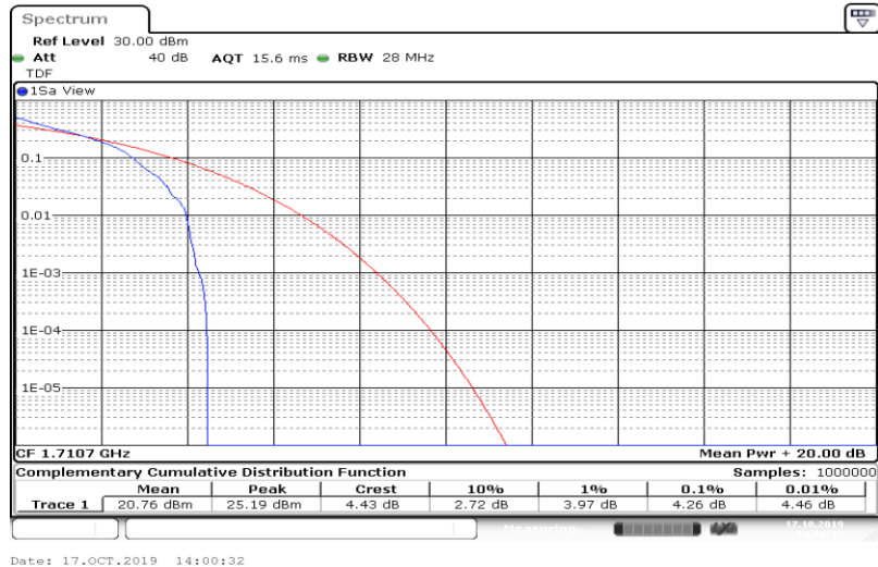
Band4-1.4MHz-QPSK-19957-6RB#0
