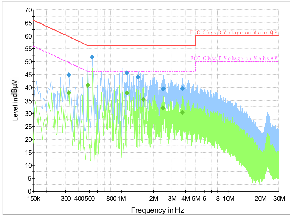
Fig.B.11.1 AC Powerline Conducted Emission- Bluetooth
