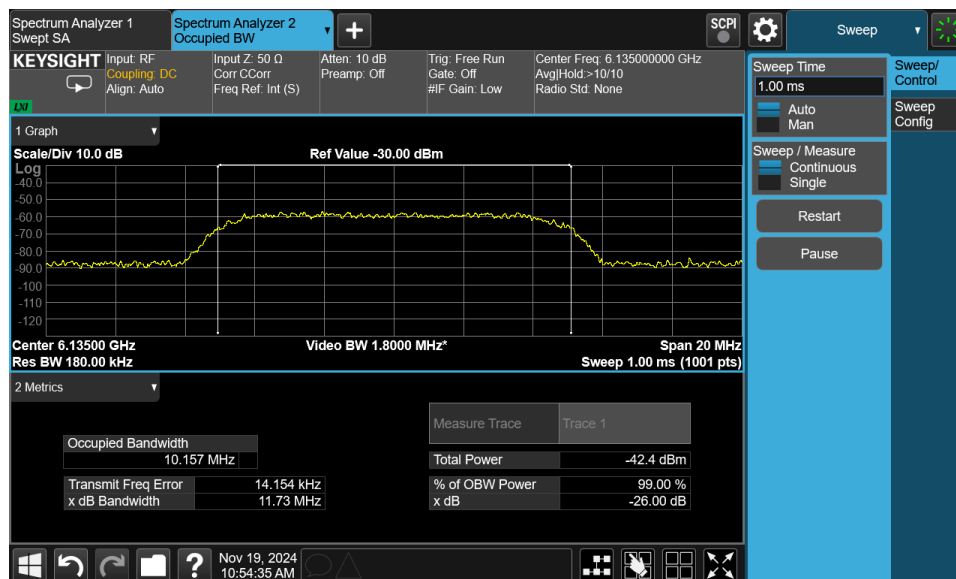
Plot 1: AWGN Signal BW Details
