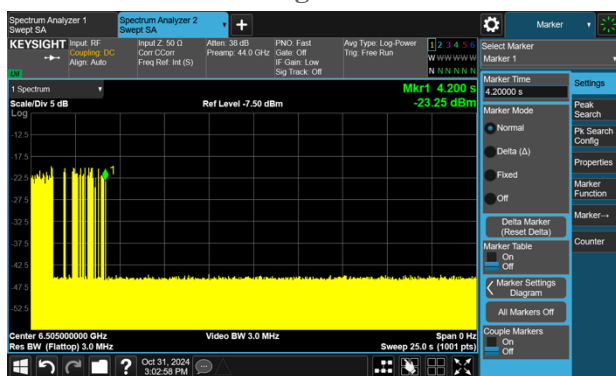
Plot 6: AWGN Signal Detection 160MHz
