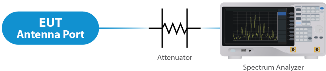
Figure 2: Direct Connect at the Antenna Port Test Radiated Emissions
