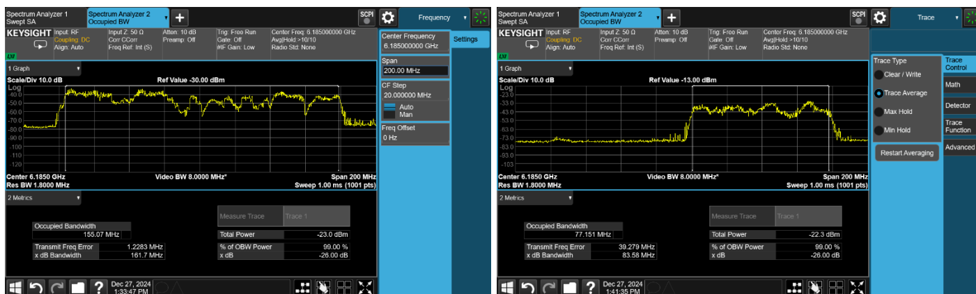
Plot 3: EUT 160MHz Transmission and Bandwidth Reduction (Example)
