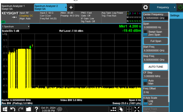
Plot 7: AWGN Signal Detection 160MHz
