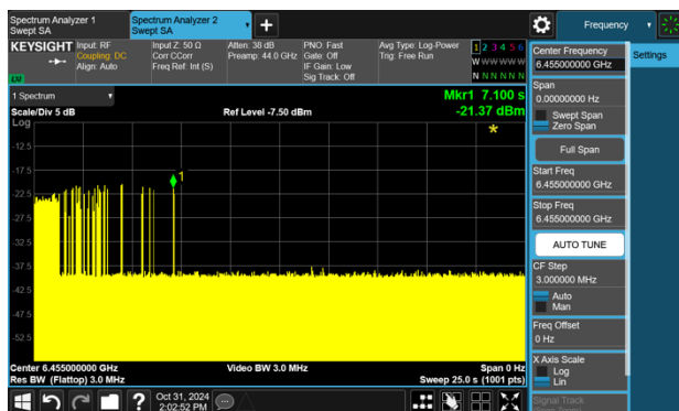
Plot 4: AWGN Signal Detection 20MHz
