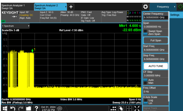
Plot 5: AWGN Signal Detection 160MHz
