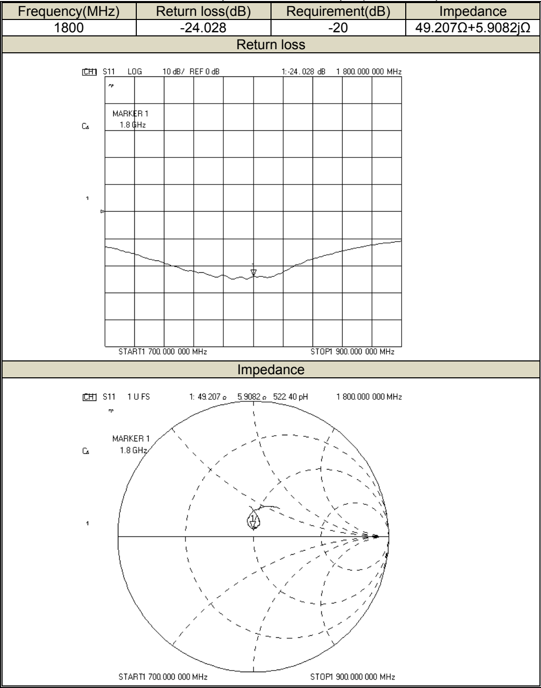
Return Loss and Impedance in Head liquid(2020-02-28)
