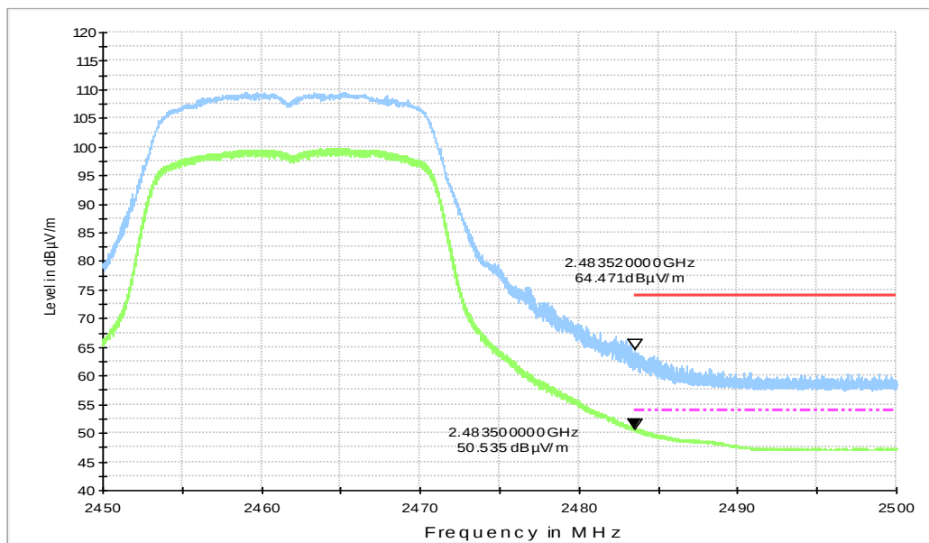
Fig.B.6.2.10 Transmitter Spurious Emission - Radiated (Power): 802.11n-HT20, ch11, 2.45 GHz - 2.50GHz
