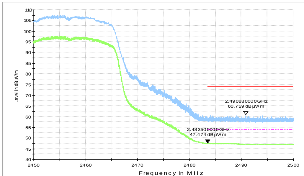
Fig.B.6.2.9 Transmitter Spurious Emission - Radiated (Power): 802.11n-HT20, ch10, 2.45 GHz - 2.50GHz
