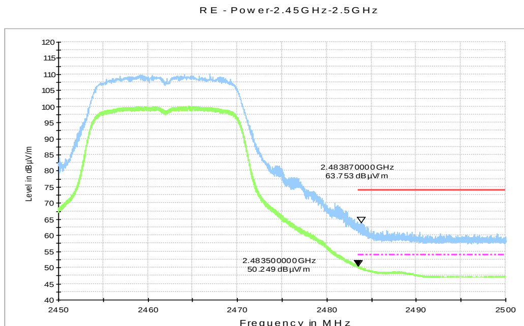
Fig.B.6.2.6 Transmitter Spurious Emission - Radiated (Power): 802.11g, ch11, 2.45 GHz - 2.50GHz
