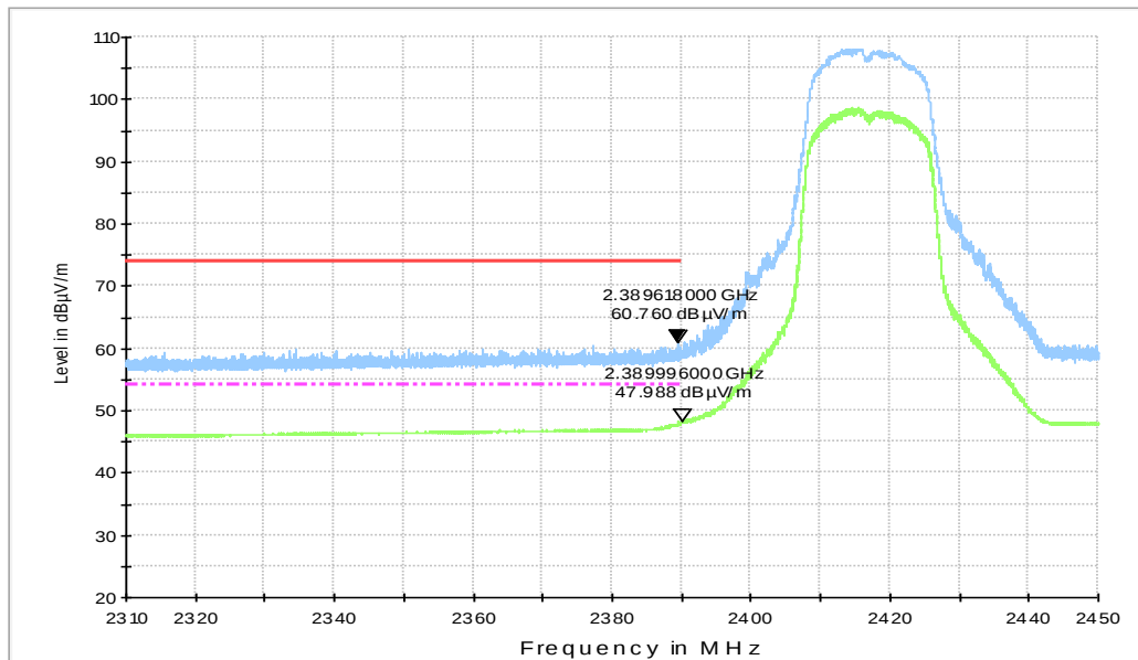
Fig.B.6.2.8 Transmitter Spurious Emission - Radiated (Power): 802.11n-HT20, ch2, 2.31GHz - 2.45GHz
