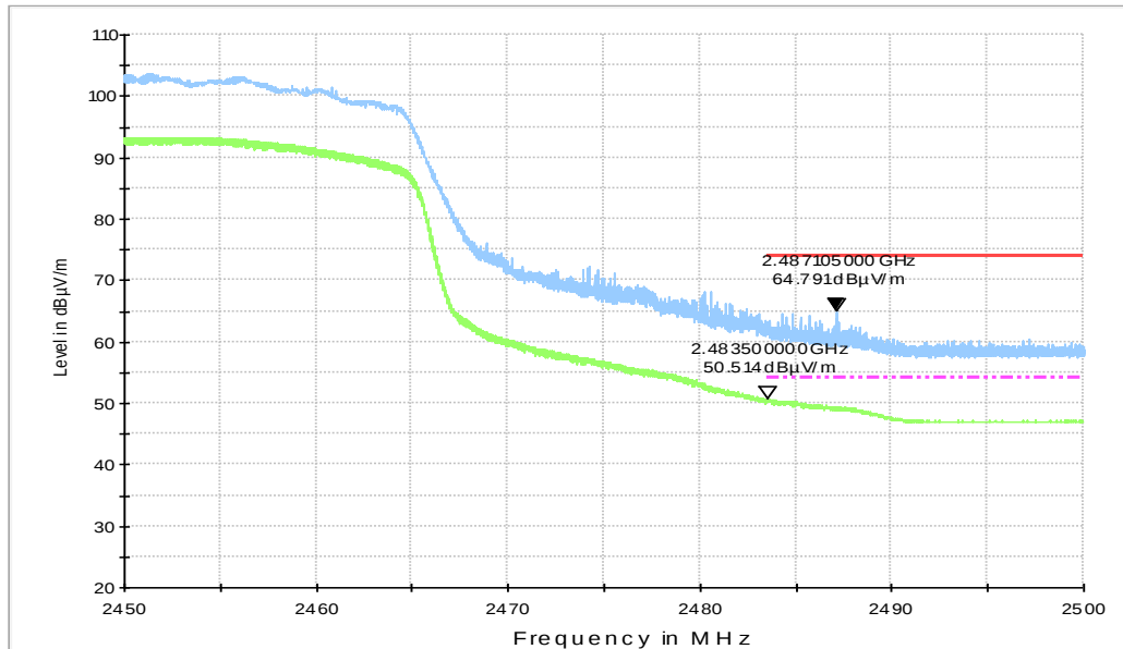
Fig.B.6.2.15 Transmitter Spurious Emission - Radiated (Power): 802.11n-HT40, ch8, 2.45 GHz - 2.50GHz
