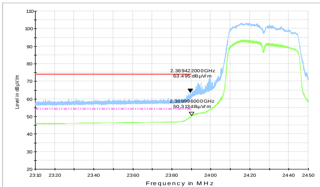
Fig.B.6.2.12 Transmitter Spurious Emission - Radiated (Power): 802.11n-HT40, ch4, 2.31GHz - 2.45GHz
