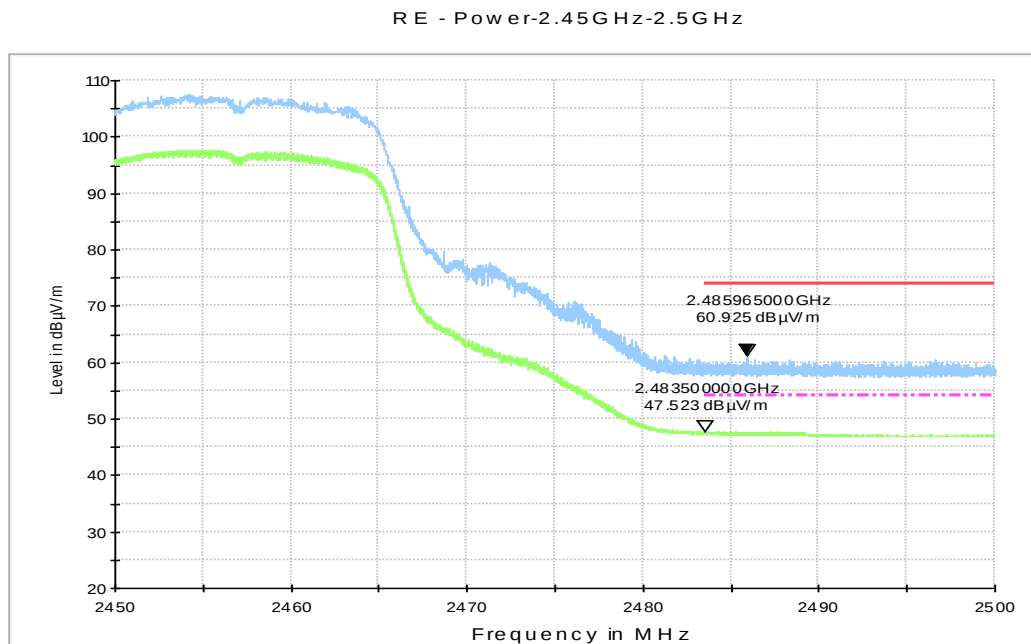
Fig.B.6.2.5 Transmitter Spurious Emission - Radiated (Power): 802.11g, ch10, 2.45 GHz - 2.50GHz
