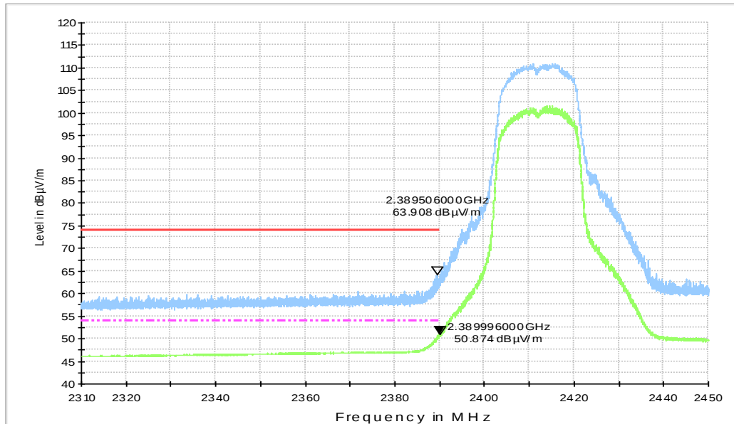
Fig.B.6.2.7 Transmitter Spurious Emission - Radiated (Power): 802.11n-HT20, ch1, 2.31GHz - 2.45GHz
