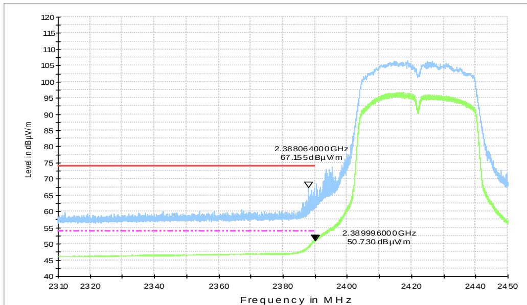
Fig.B.6.2.11 Transmitter Spurious Emission - Radiated (Power): 802.11n-HT40, ch3, 2.31GHz - 2.45GHz
