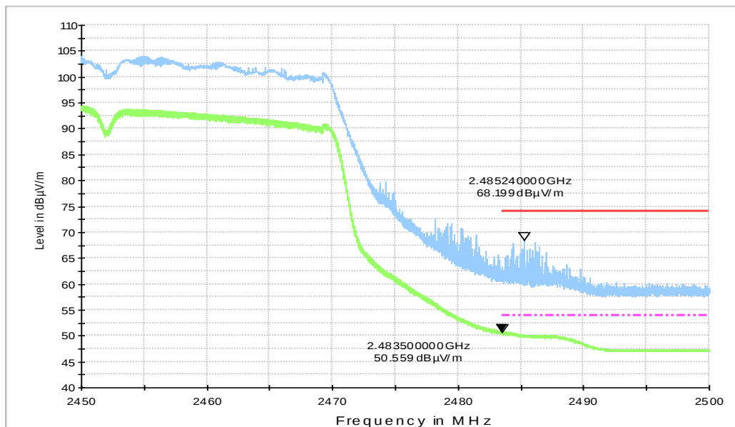
Fig.B.6.2.16 Transmitter Spurious Emission - Radiated (Power): 802.11n-HT40, ch9, 2.45 GHz - 2.50GHz
