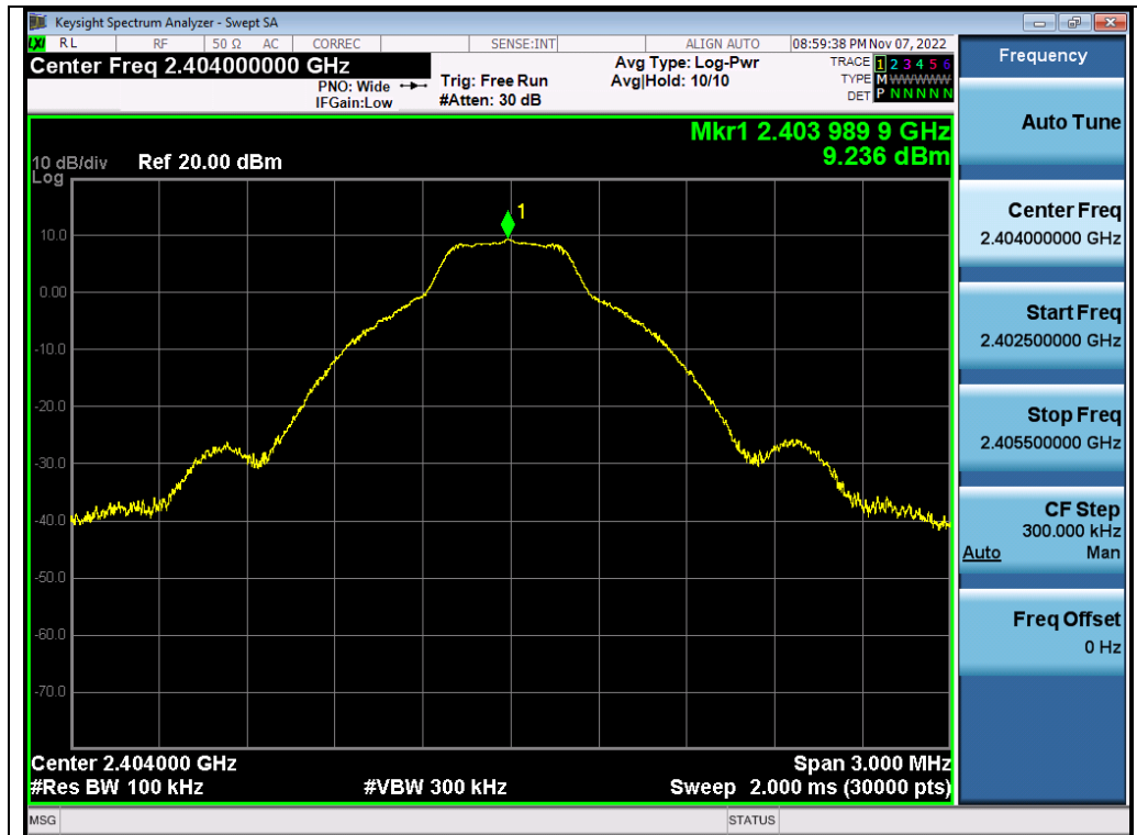
Test_Graph_2.4G_ANT2_2404_1Mbps_Reference Level
