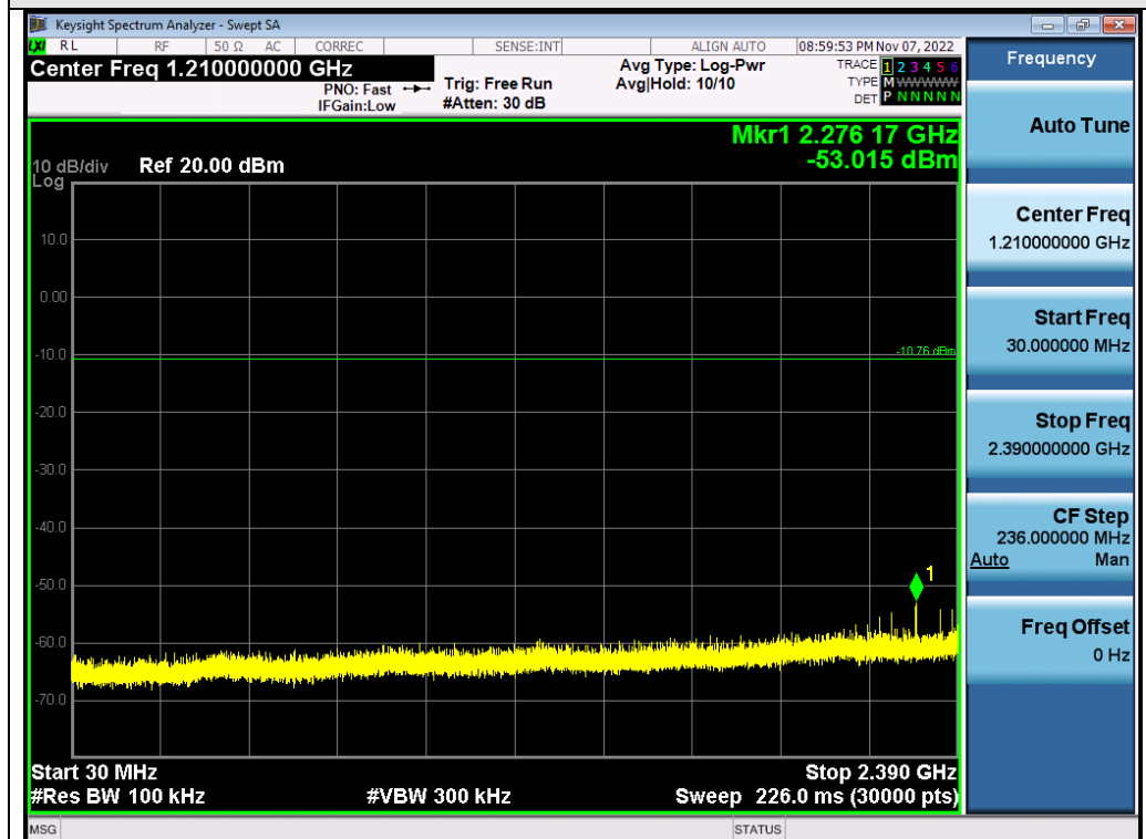
Test_Graph_2.4G_ANT2_2404_1Mbps_Lower Band Emissions
