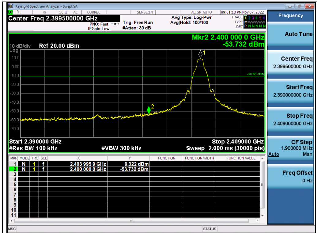
Test_Graph_2.4G_ANT2_2404_1Mbps_Lower Band Edge Emissions
