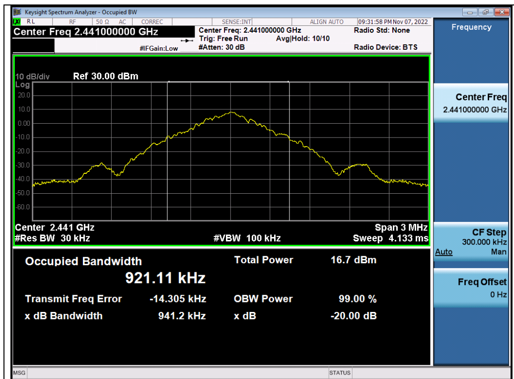
Test_Graph_2.4G_ANT2_2441_1Mbps_OBW
