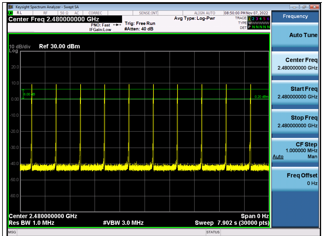
Test_Graph_2.4G_HOP_ANT2_NA_1Mbps_2480_Number of Burst
