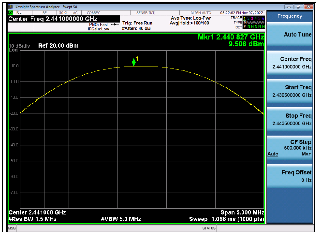
Test_Graph_2.4G_ANT1_2441_1Mbps_Peak Power
