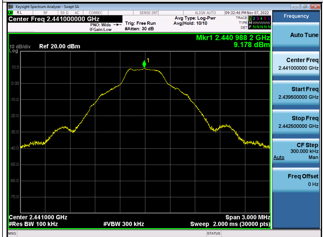
Test_Graph_2.4G_ANT2_2441_1Mbps_Reference Level
