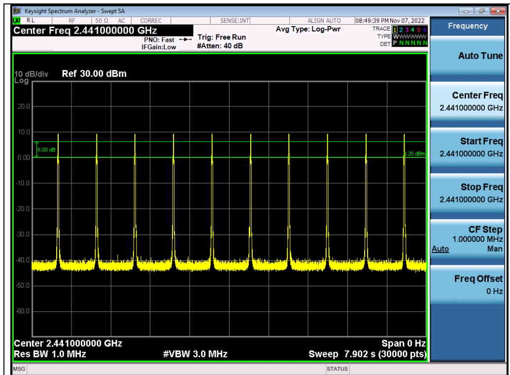
Test_Graph_2.4G_HOP_ANT2_NA_1Mbps_2441_Number of Burst
