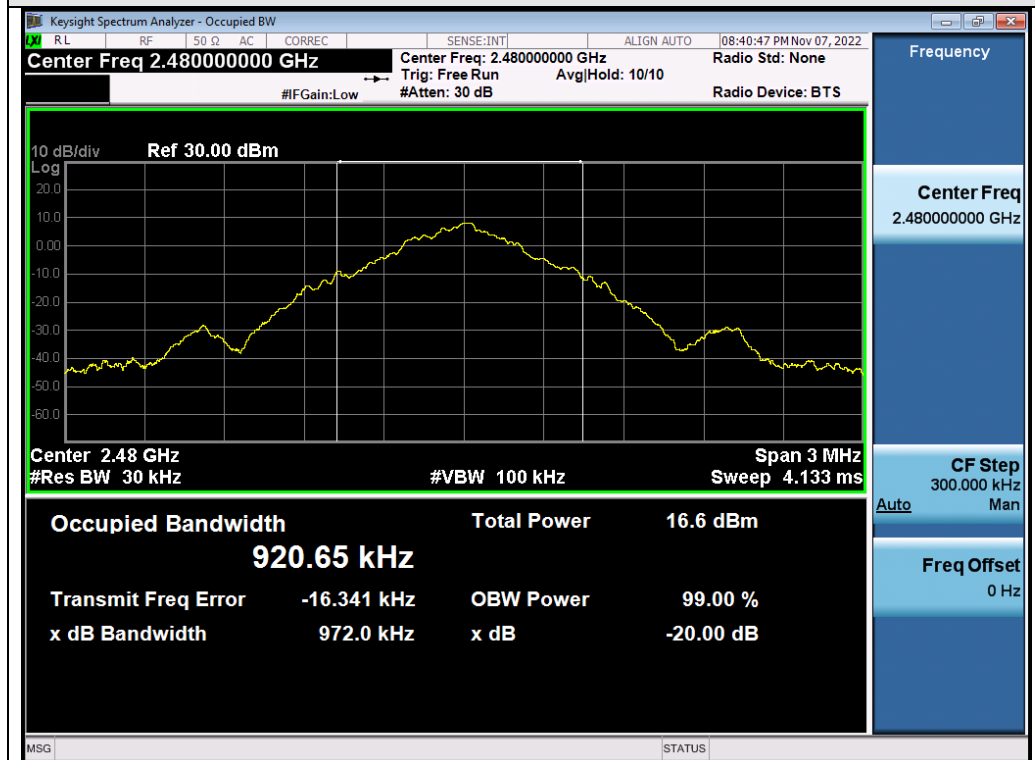
Test_Graph_2.4G_ANT2_2480_1Mbps_OBW
