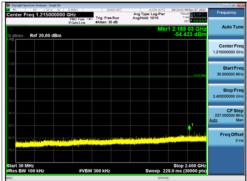
Test_Graph_2.4G_ANT2_2441_1Mbps_Lower Band Emissions
