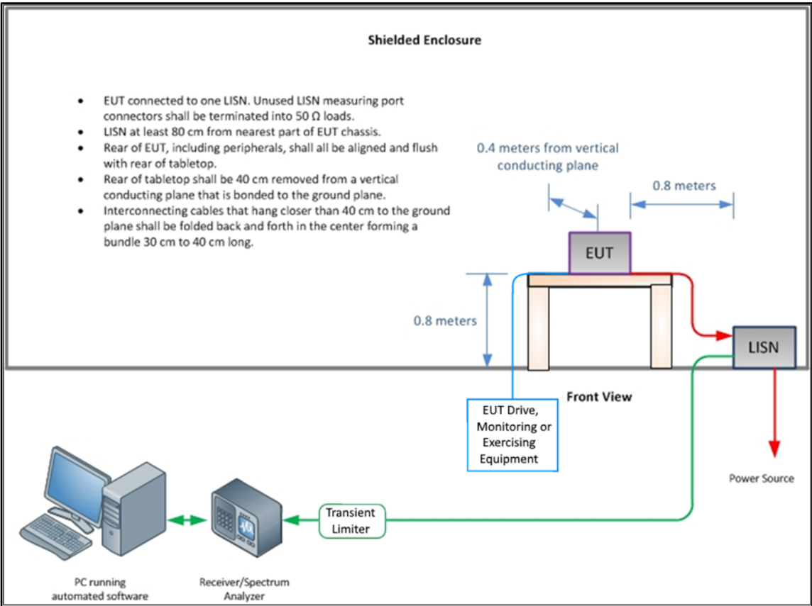
Figure 1 - Conducted Disturbance
