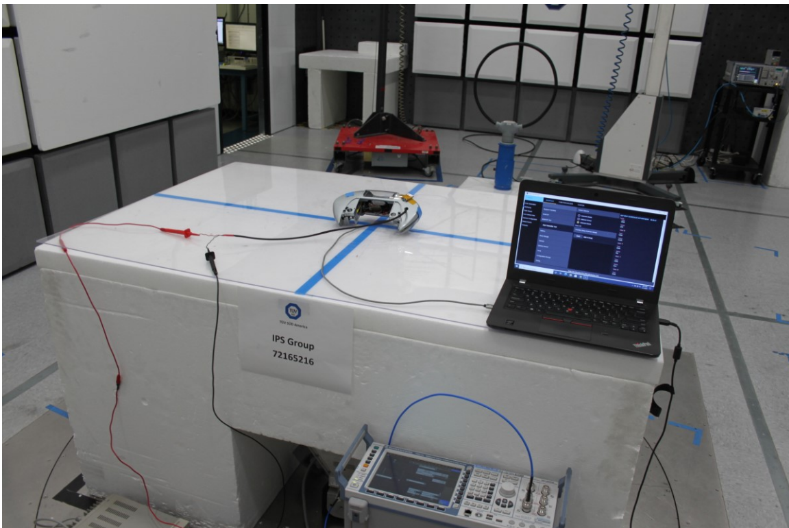
Radiated Emissions 9 kHz to 30 MHz
