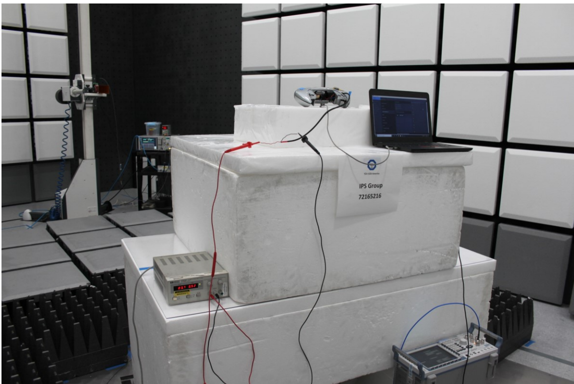
Radiated Emissions Above 18 GHz to 26 GHz
