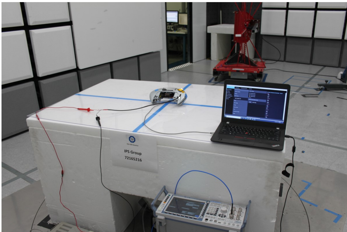
Radiated Emissions 30 MHz to 1 GHz
