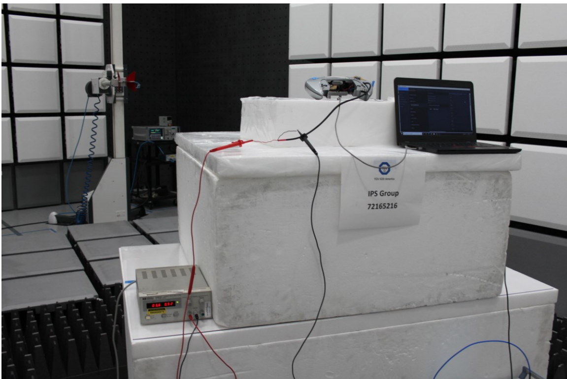
Radiated Emissions 1 GHz to 18 GHz
