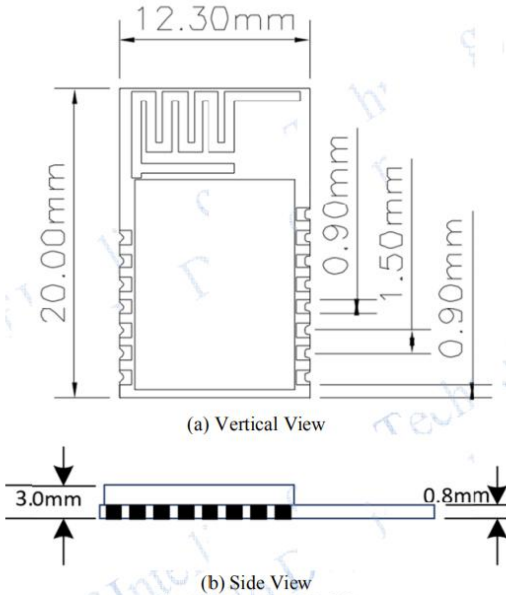
Fig. 3.4 Size for ESP-M1
