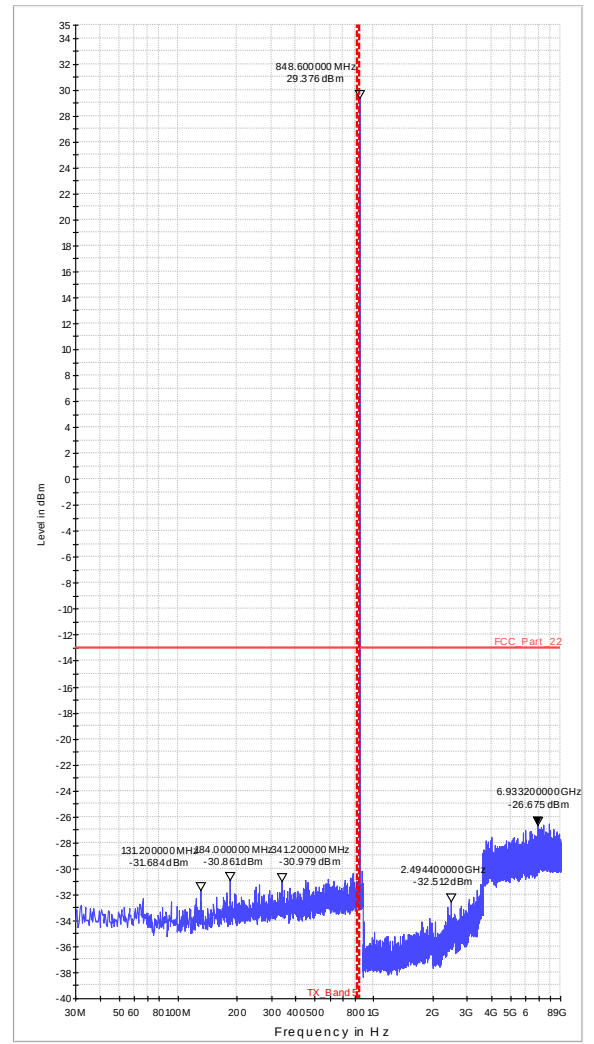
Diagram 36.18_RSE_Ch251_EGPRS_Sweep2
