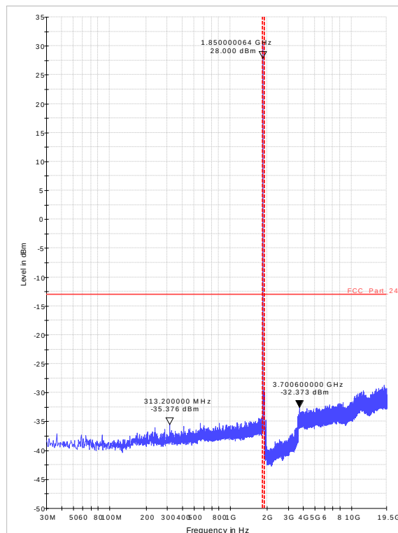
Diagram 36.21_RSE_Ch512_GPRS_Sweep2
