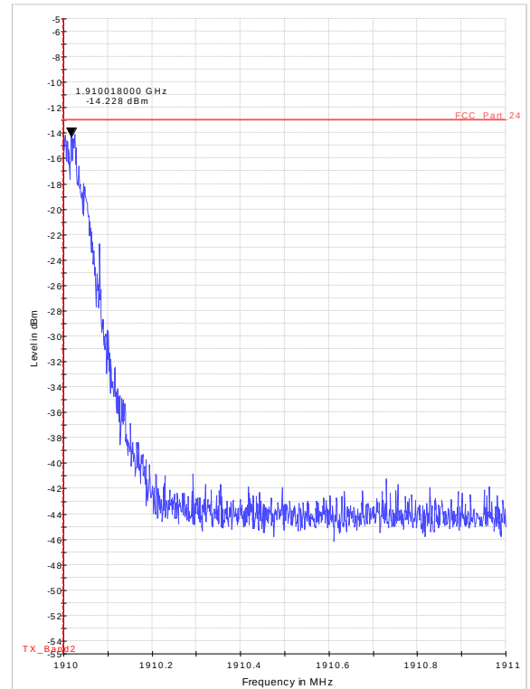
Diagram 37.11_BE_Ch810_GPRS_PK
