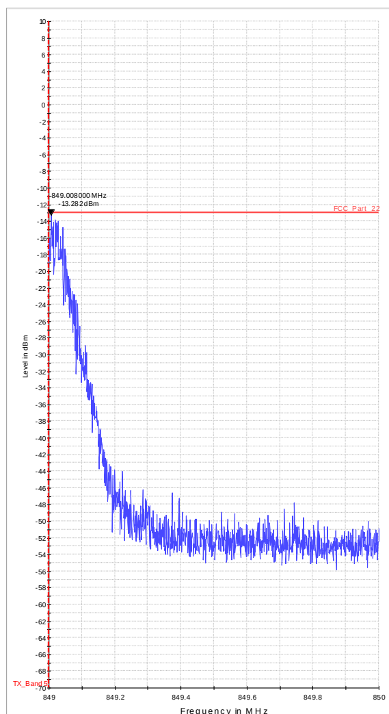
Diagram 37.04_BE_Ch251_GPRS
