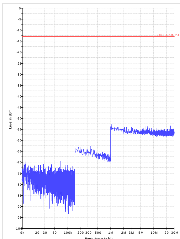
Diagram 36.20_RSE_Ch512_GPRS_Sweep1
