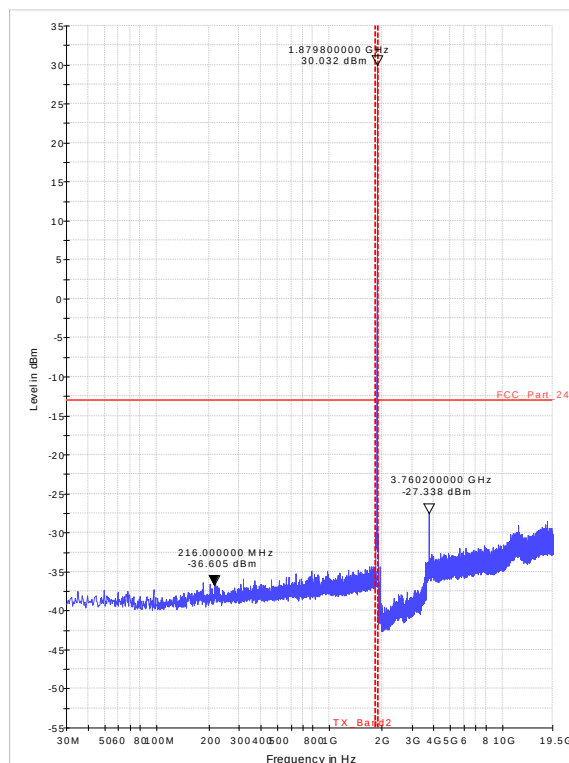
Diagram 36.23_RSE_Ch661_GPRS_Sweep2
