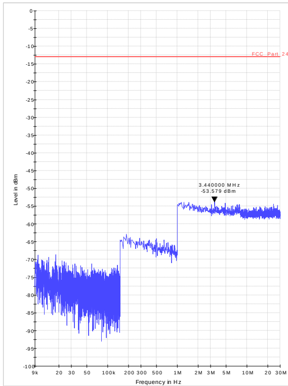
Diagram 36.28_RSE_Ch661_EGPRS_Sweep1
