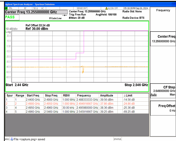
n41 50M DFT-s-OFDM BPSK Edge_1RB_Left Low
