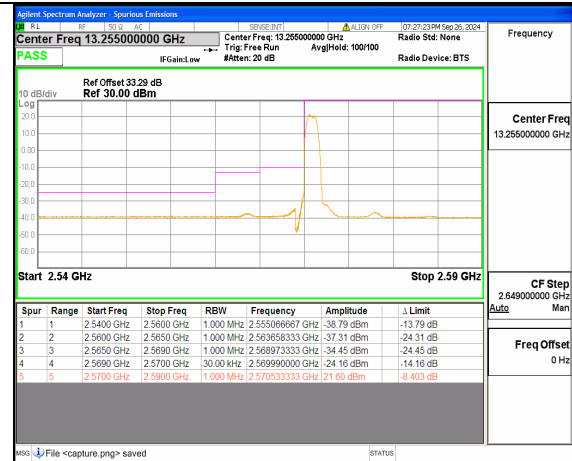
n38 15M DFT-s-OFDM BPSK Edge_1RB_Left Low
