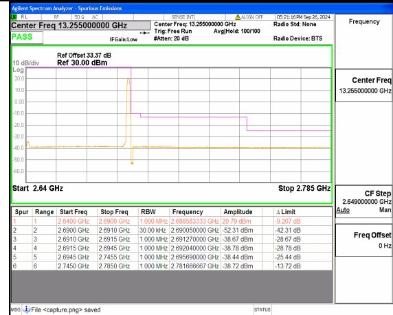
n41 50M DFT-s-OFDM BPSK Edge_1RB_Right High
