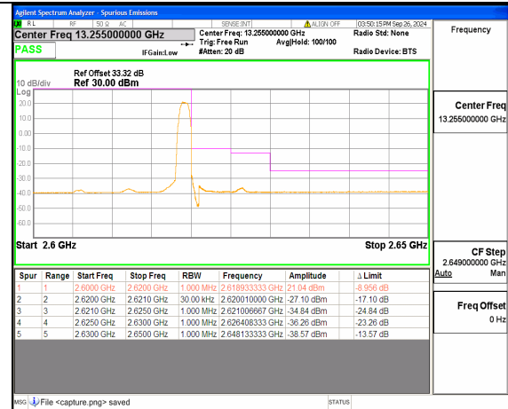
n38 15M DFT-s-OFDM QPSK Edge_1RB_Right High
