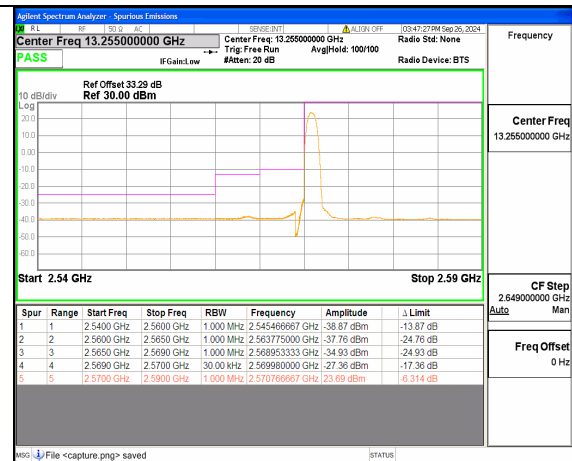
n38 15M DFT-s-OFDM QPSK Edge_1RB_Left Low
