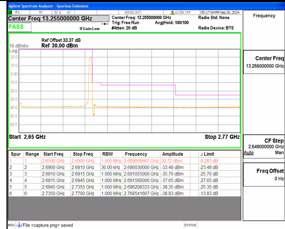
n41 40M DFT-s-OFDM QPSK Edge_1RB_Right High
