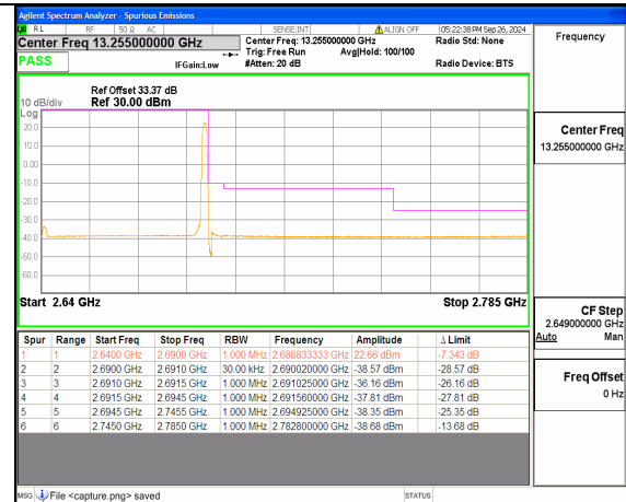
n41 50M DFT-s-OFDM QPSK Edge_1RB_Right High
