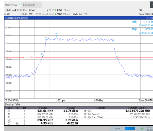
1-N26-824-849--15-5-M-9-CP-256QAM-Outer_Full-2 5@0-Ant0-4.473-4.950-≤5-PASS
