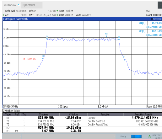
1-N26-824-849--15-5-M-8-CP-64QAM-Outer_Full-25 @0-Ant0-4.479-5.070-≤5-PASS
