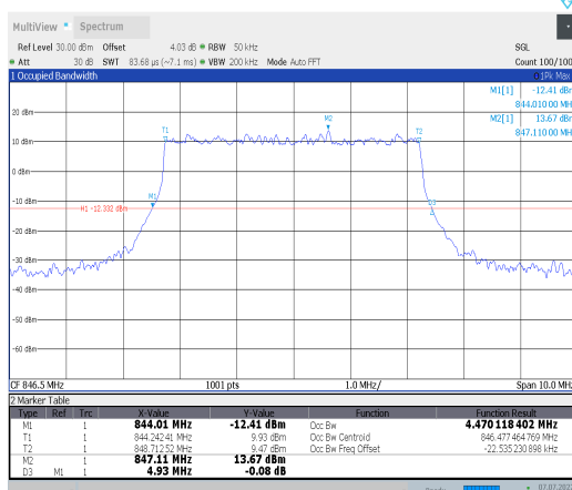
1-N26-824-849--15-5-H-1-DFT-QPSK-Outer_Full-25 @0-Ant0-4.47-4.930-≤5-PASS
