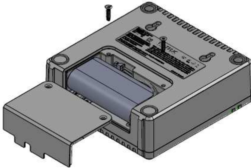
Figure 6: Battery Installation
