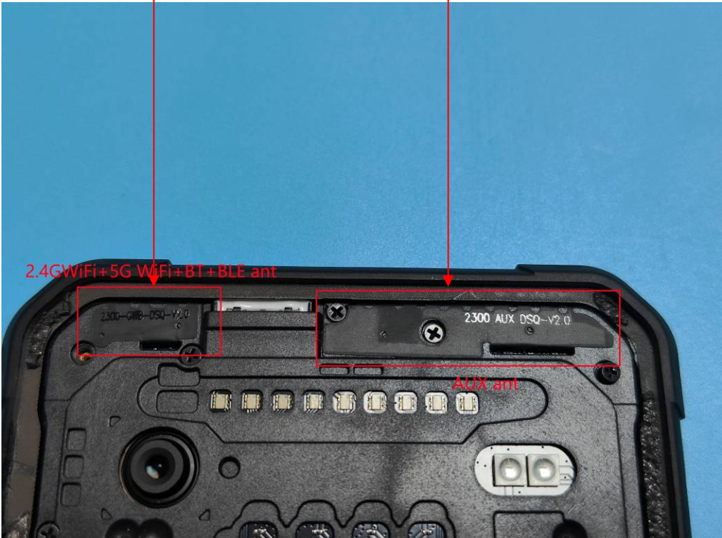
BT/Wi-Fi Ant
