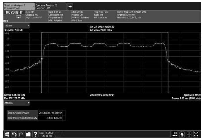
Figure 22: 16QAM 15MHz B.W.; 2117.5MHz, 15kHz
