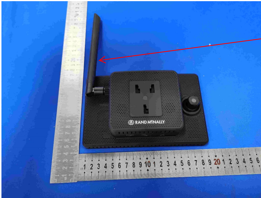
FM antenna
