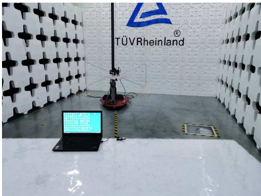
Photograph 2: Set-up photo for Radiated Emission, Below 1GHz
