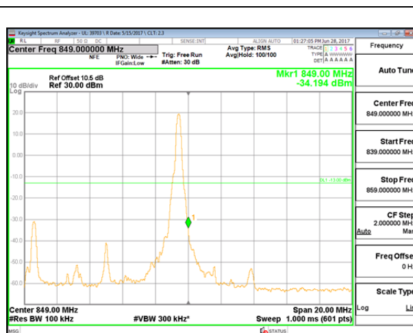
LTE B5 10MHz 16QAM High Channel 1RB
