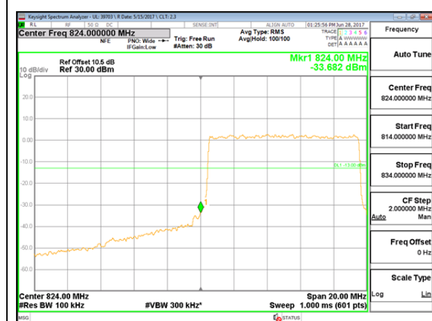
LTE B5 10MHz 16QAM Low Channel FRB
