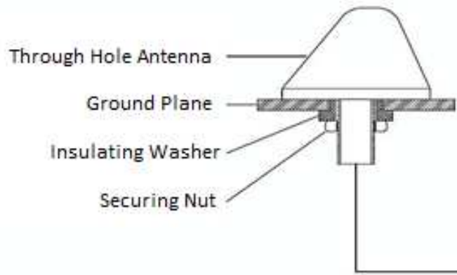
Vertical cut of a QF036 after installation
