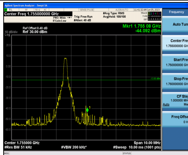
Band4-15MHz-16QAM-20325-1-5-High--44.09-PASS
