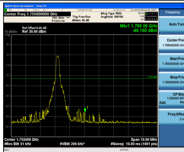
Band4-20MHz-16QAM-20300-1-5-High--46.15-PASS
