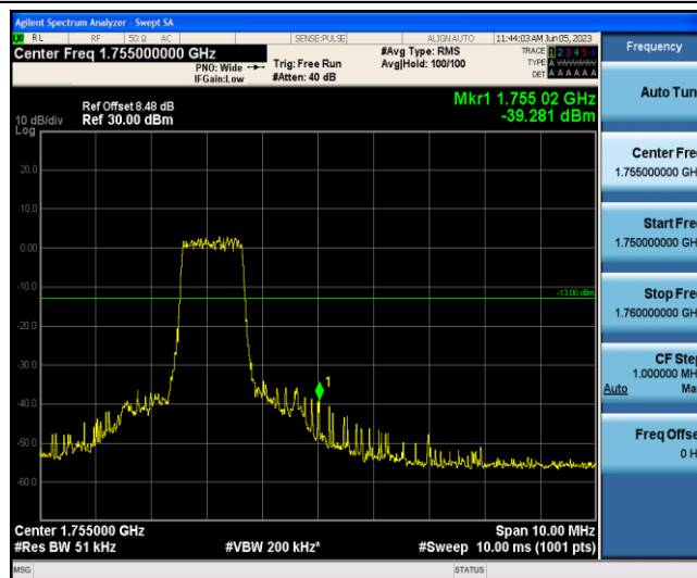
Band4-20MHz-QPSK-20300-6-0-High--39.28-PASS
