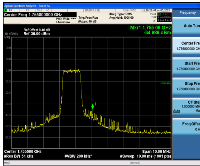
Band4-10MHz-QPSK-20350-6-0-High--34.99-PASS
