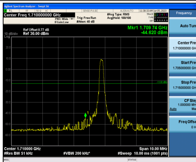
Band4-10MHz-16QAM-20000-1-0-Low--44.62-PASS
