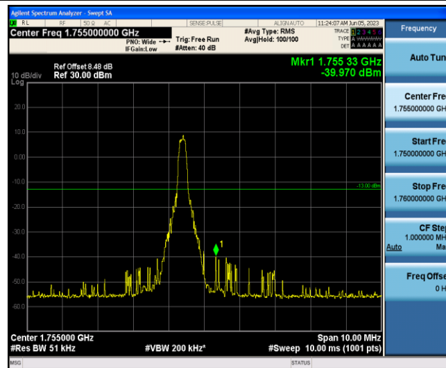
Band4-1.4MHz-16QAM-20393-1-5-High--39.97-PASS
