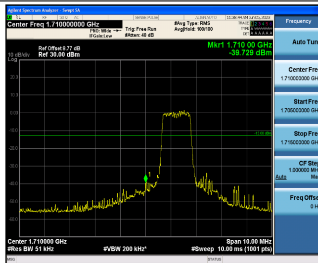
Band4-10MHz-QPSK-20000-6-0-Low--39.73-PASS
