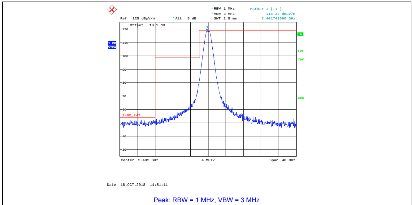
Plot 5.4.4.2.1. Band-Edge Radiated Emissions, Lower Band-edge Rx Antenna in Vertical Polarization, GFSK Modulation, 1 Mbps, Power Setting 200, Ch 37, 2402 MHz
