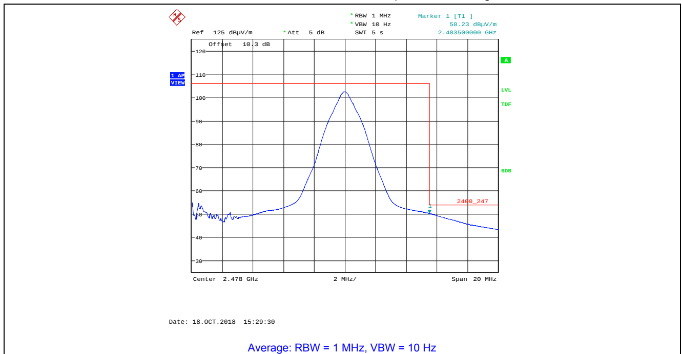
Plot 5.4.4.2.20. Band-Edge Radiated Emissions, Higher Band-edge Rx Antenna in Vertical Polarization, GFSK Modulation, 2 Mbps, Power Setting 200, Ch 36, 2478 MHz
