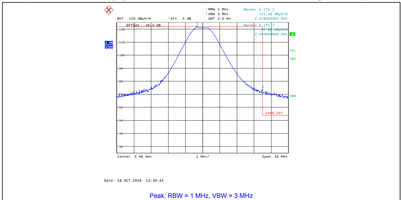
Plot 5.4.4.2.10. Band-Edge Radiated Emissions, Higher Band-edge Rx Antenna in Horizontal Polarization, GFSK Modulation, 1 Mbps, Power Setting 200, Ch 39, 2480 MHz Applied Maximum 20 dB Duty Cycle Correction Factor Applied to 72.09 dB \mu V/m Peak, Average is 52.09 dB \mu V/m
