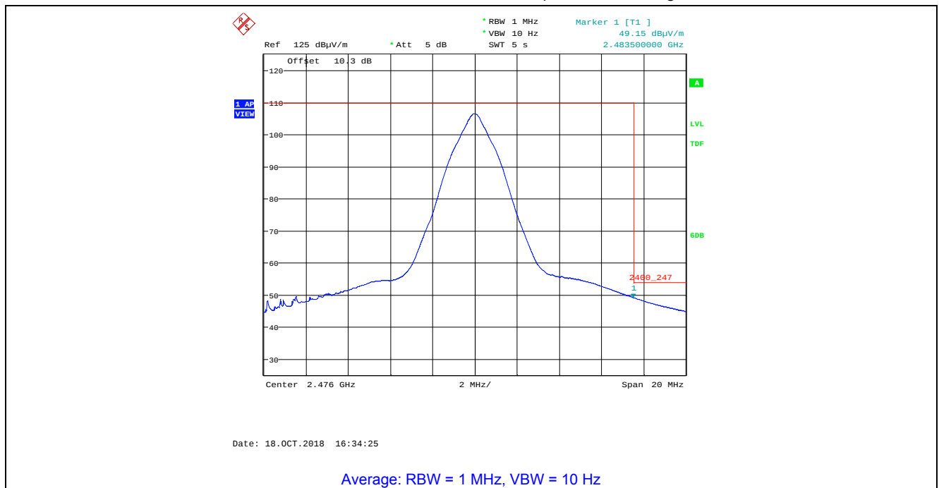
Plot 5.4.4.2.16. Band-Edge Radiated Emissions, Higher Band-edge Rx Antenna in Vertical Polarization, GFSK Modulation, 2 Mbps, Power Setting 200, Ch 35, 2476 MHz
