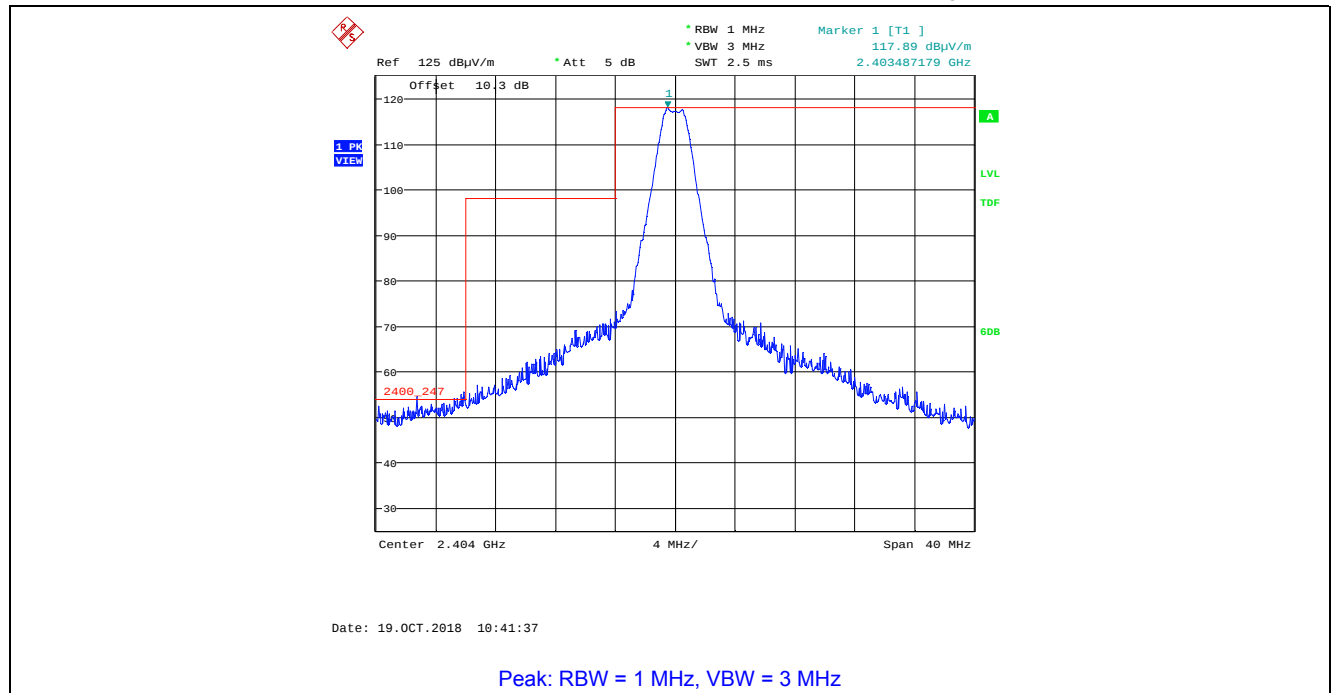
Plot 5.4.4.2.11. Band-Edge Radiated Emissions, Lower Band-edge Rx Antenna in Vertical Polarization, GFSK Modulation, 2 Mbps, Power Setting 200, Ch 00, 2404 MHz
