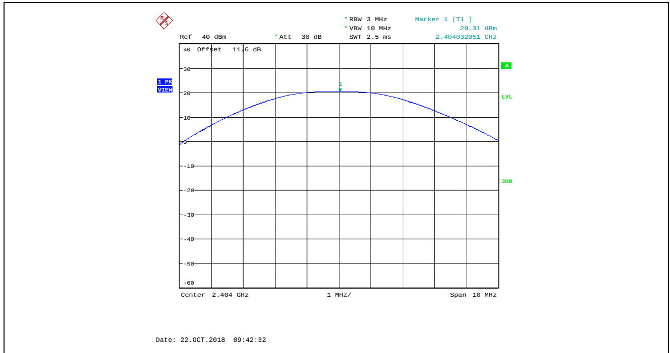
Plot 5.3.4.5. Maximum Peak Conducted Output Power, GFSK Modulation, 2 Mbps, Power Setting 200, Ch 00, 2404 MHz
