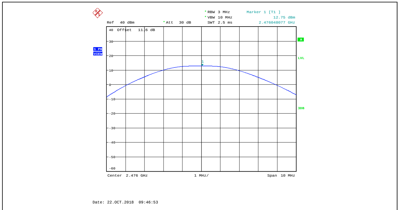
Plot 5.3.4.7. Maximum Peak Conducted Output Power, GFSK Modulation, 2 Mbps, Power Setting 200, Ch 35, 2476 MHz
