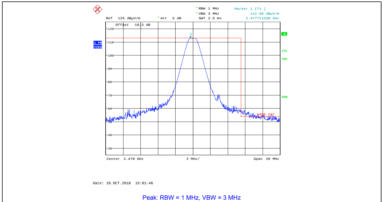
Plot 5.4.4.2.5. Band-Edge Radiated Emissions, Higher Band-edge Rx Antenna in Vertical Polarization, GFSK Modulation, 1 Mbps, Power Setting 200, Ch 36, 2478 MHz
