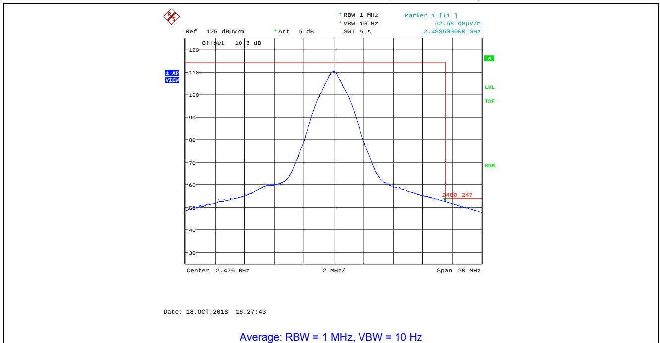
Plot 5.4.4.2.18. Band-Edge Radiated Emissions, Higher Band-edge Rx Antenna in Horizontal Polarization, GFSK Modulation, 2 Mbps, Power Setting 200, Ch 35, 2476 MHz
