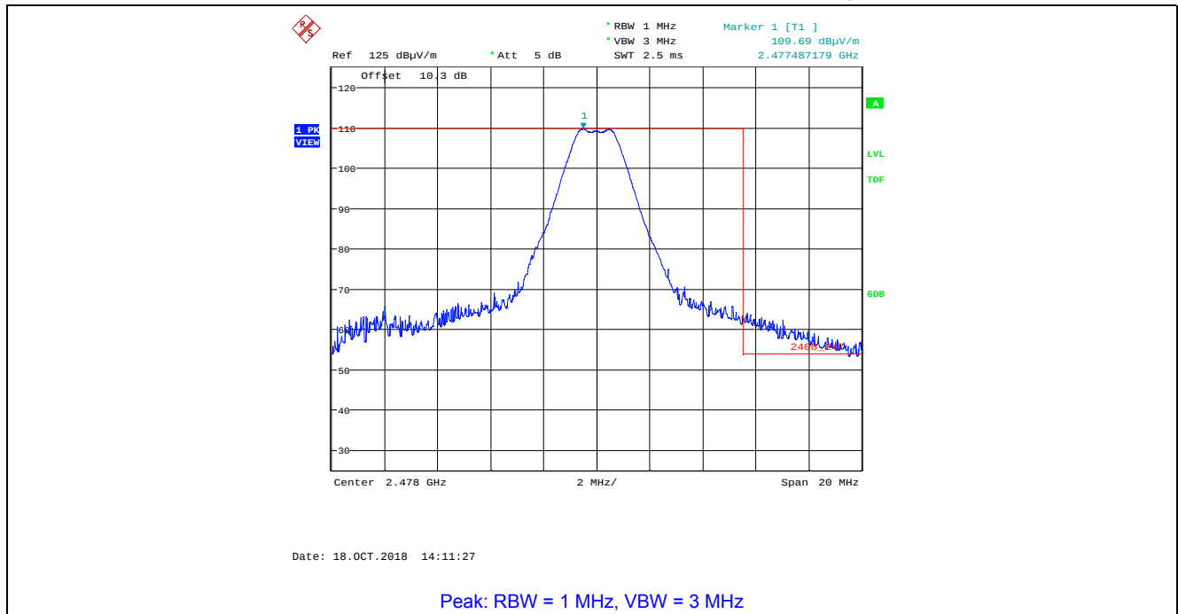
Plot 5.4.4.2.21. Band-Edge Radiated Emissions, Higher Band-edge Rx Antenna in Horizontal Polarization, GFSK Modulation, 2 Mbps, Power Setting 200, Ch 36, 2478 MHz
