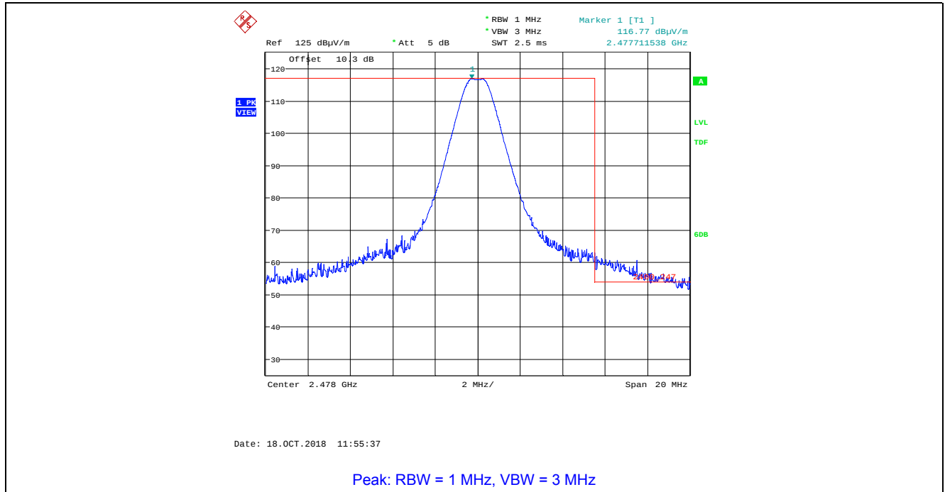
Plot 5.4.4.2.7. Band-Edge Radiated Emissions, Higher Band-edge Rx Antenna in Horizontal Polarization, GFSK Modulation, 1 Mbps, Power Setting 200, Ch 36, 2478 MHz
