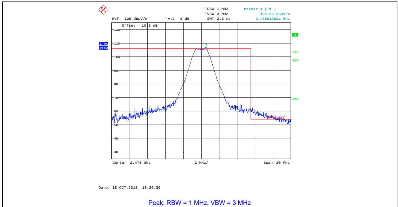
Plot 5.4.4.2.19. Band-Edge Radiated Emissions, Higher Band-edge Rx Antenna in Vertical Polarization, GFSK Modulation, 2 Mbps, Power Setting 200, Ch 36, 2478 MHz
