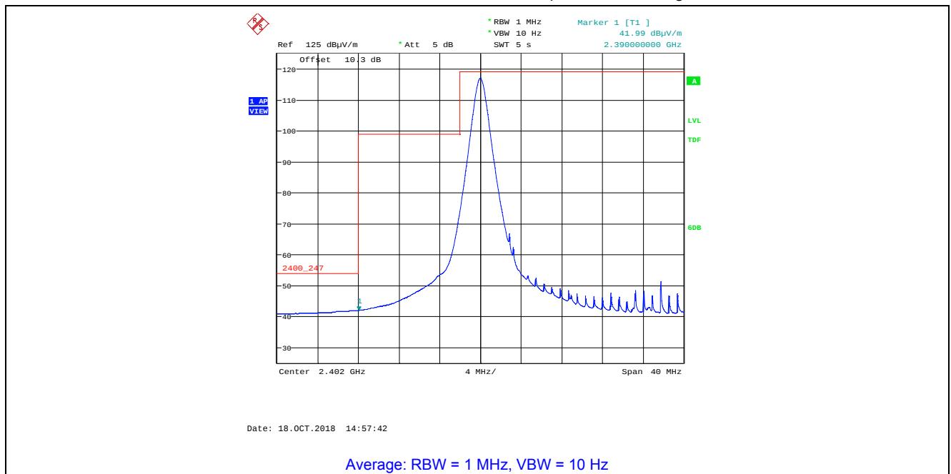
Plot 5.4.4.2.2. Band-Edge Radiated Emissions, Lower Band-edge Rx Antenna in Vertical Polarization, GFSK Modulation, 1 Mbps, Power Setting 200, Ch 37, 2402 MHz
