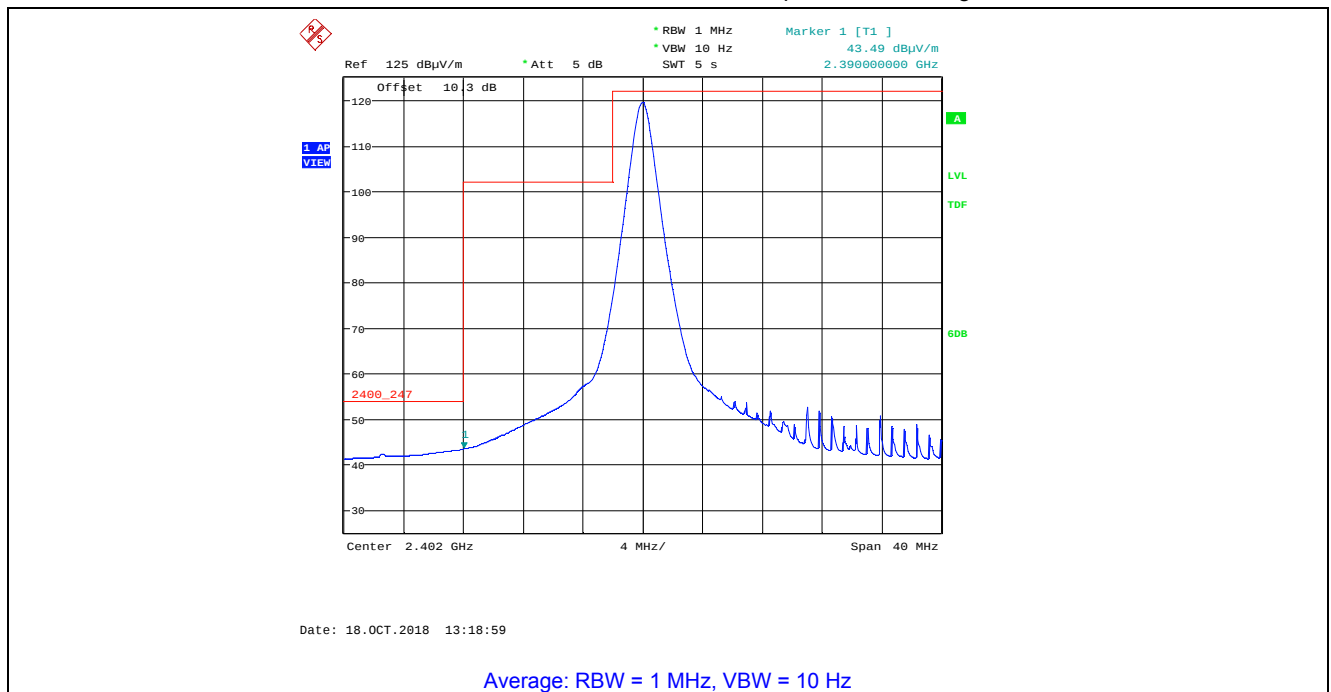
Plot 5.4.4.2.4. Band-Edge Radiated Emissions, Lower Band-edge Rx Antenna in Horizontal Polarization, GFSK Modulation, 1 Mbps, Power Setting 200, Ch 37, 2402 MHz
