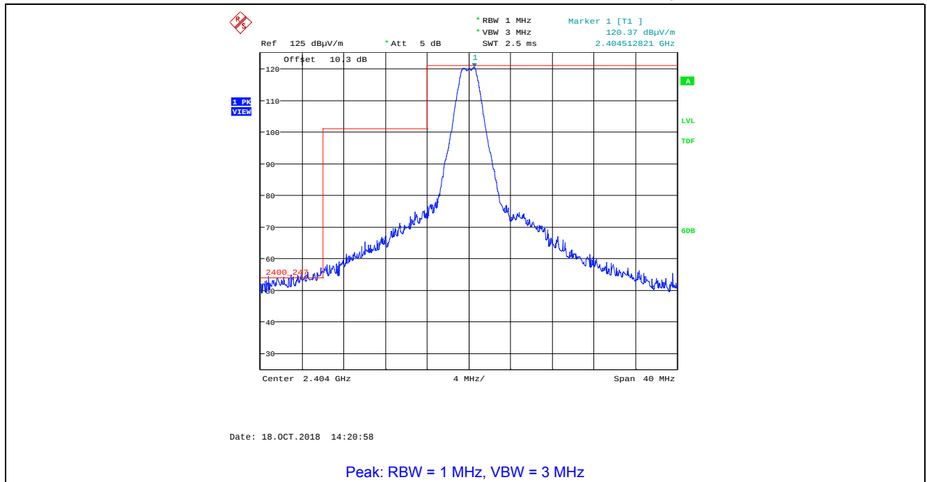
Plot 5.4.4.2.13. Band-Edge Radiated Emissions, Lower Band-edge Rx Antenna in Horizontal Polarization, GFSK Modulation, 2 Mbps, Power Setting 200, Ch 00, 2404 MHz
