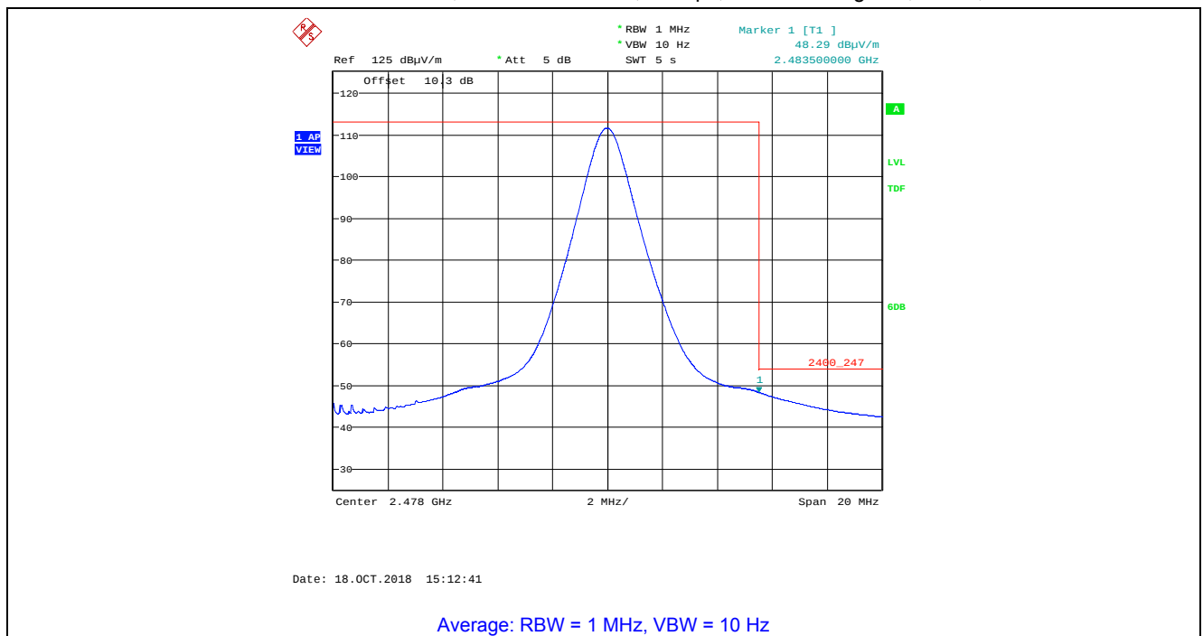
Plot 5.4.4.2.6. Band-Edge Radiated Emissions, Higher Band-edge Rx Antenna in Vertical Polarization, GFSK Modulation, 1 Mbps, Power Setting 200, Ch 36, 2478 MHz
