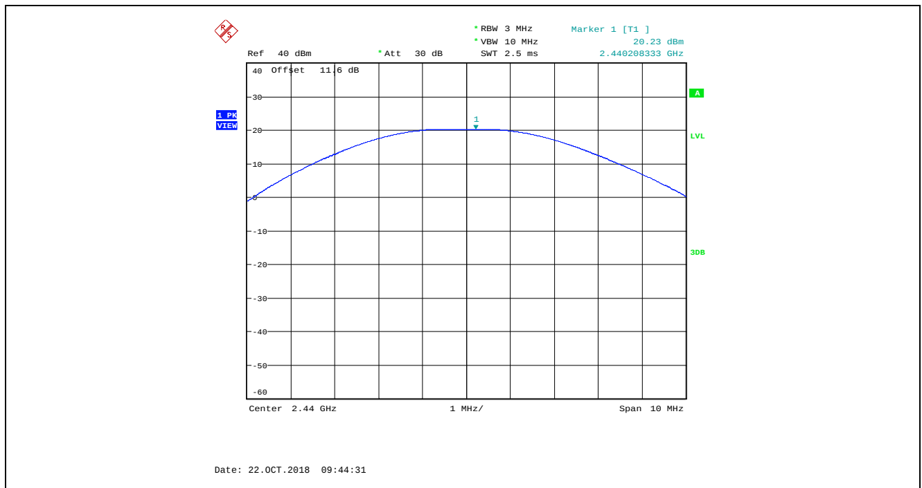
Plot 5.3.4.6. Maximum Peak Conducted Output Power, GFSK Modulation, 2 Mbps, Power Setting 200, Ch 17, 2440 MHz
