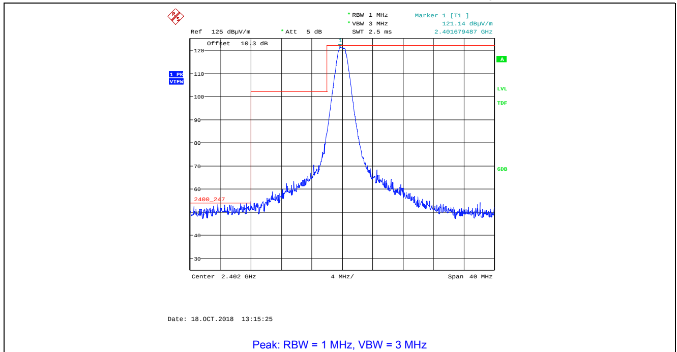
Plot 5.4.4.2.3. Band-Edge Radiated Emissions, Lower Band-edge Rx Antenna in Horizontal Polarization, GFSK Modulation, 1 Mbps, Power Setting 200, Ch 37, 2402 MHz
