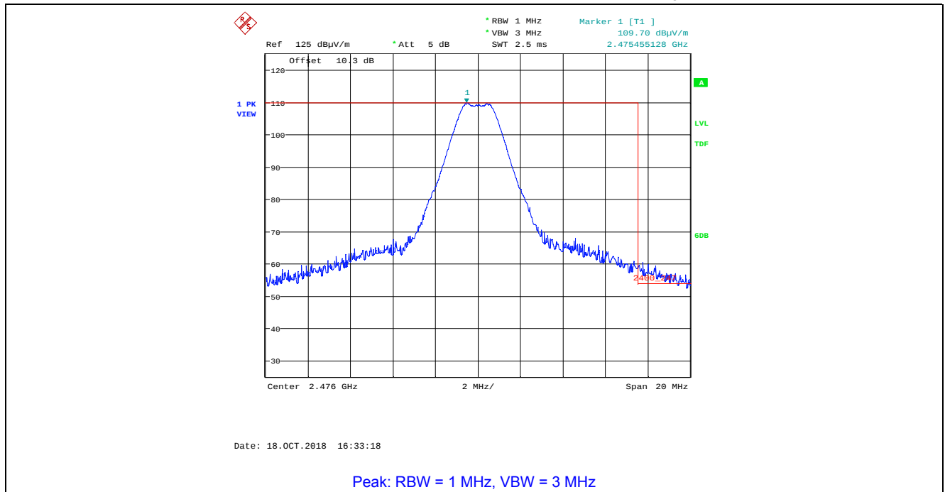
Plot 5.4.4.2.15. Band-Edge Radiated Emissions, Higher Band-edge Rx Antenna in Vertical Polarization, GFSK Modulation, 2 Mbps, Power Setting 200, Ch 35, 2476 MHz
