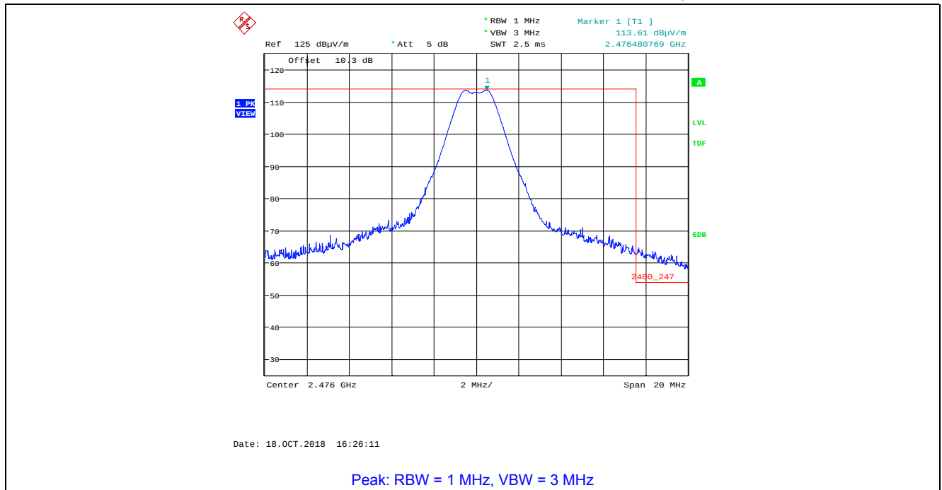
Plot 5.4.4.2.17. Band-Edge Radiated Emissions, Higher Band-edge Rx Antenna in Horizontal Polarization, GFSK Modulation, 2 Mbps, Power Setting 200, Ch 35, 2476 MHz
