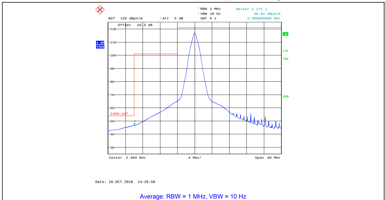
Plot 5.4.4.2.14. Band-Edge Radiated Emissions, Lower Band-edge Rx Antenna in Horizontal Polarization, GFSK Modulation, 2 Mbps, Power Setting 200, Ch 00, 2404 MHz
