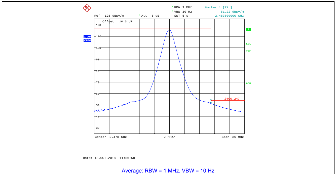
Plot 5.4.4.2.8. Band-Edge Radiated Emissions, Higher Band-edge Rx Antenna in Horizontal Polarization, GFSK Modulation, 1 Mbps, Power Setting 200, Ch 36, 2478 MHz
