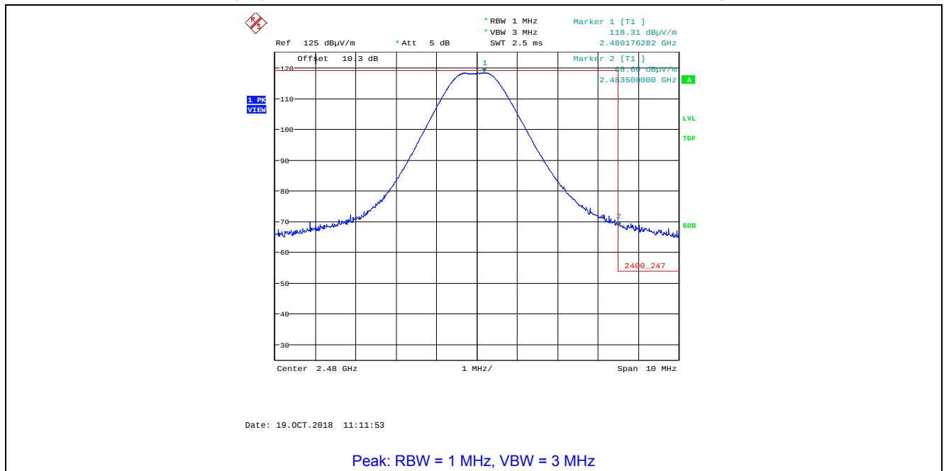
Plot 5.4.4.2.9. Band-Edge Radiated Emissions, Higher Band-edge Rx Antenna in Vertical Polarization, GFSK Modulation, 1 Mbps, Power Setting 200, Ch 39, 2480 MHz Maximum 20 dB Duty Cycle Correction Factor Applied to 68.66 dB \mu V/m Peak, Average is 48.66 dB \mu V/m
