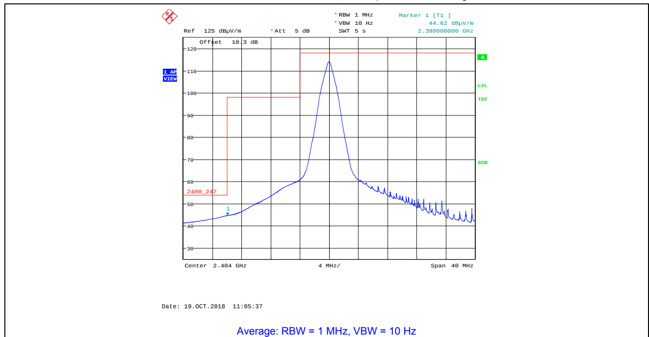
Plot 5.4.4.2.12. Band-Edge Radiated Emissions, Lower Band-edge Rx Antenna in Vertical Polarization, GFSK Modulation, 2 Mbps, Power Setting 200, Ch 00, 2404 MHz
