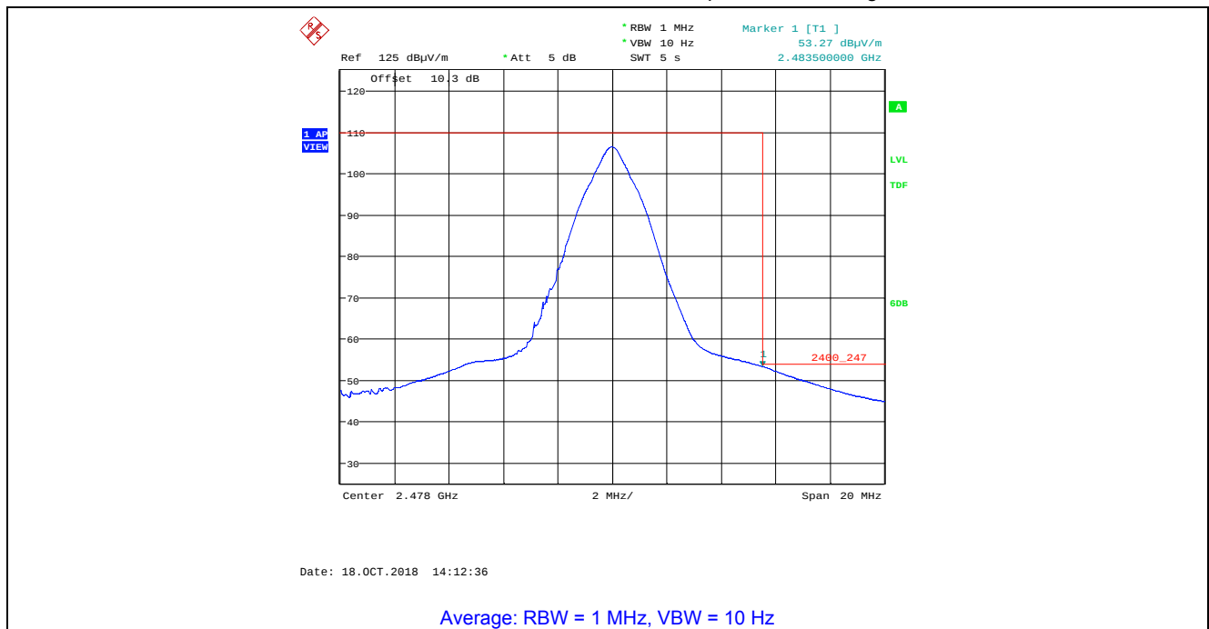
Plot 5.4.4.2.22. Band-Edge Radiated Emissions, Higher Band-edge Rx Antenna in Horizontal Polarization, GFSK Modulation, 2 Mbps, Power Setting 200, Ch 36, 2478 MHz
