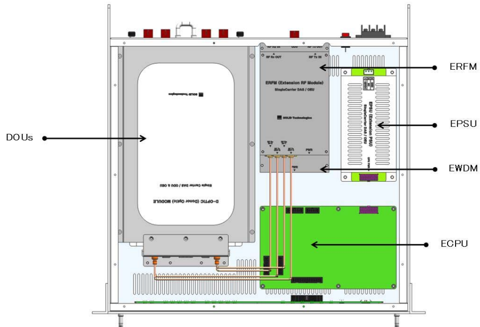
Figure 4.22 – OEU internal view
