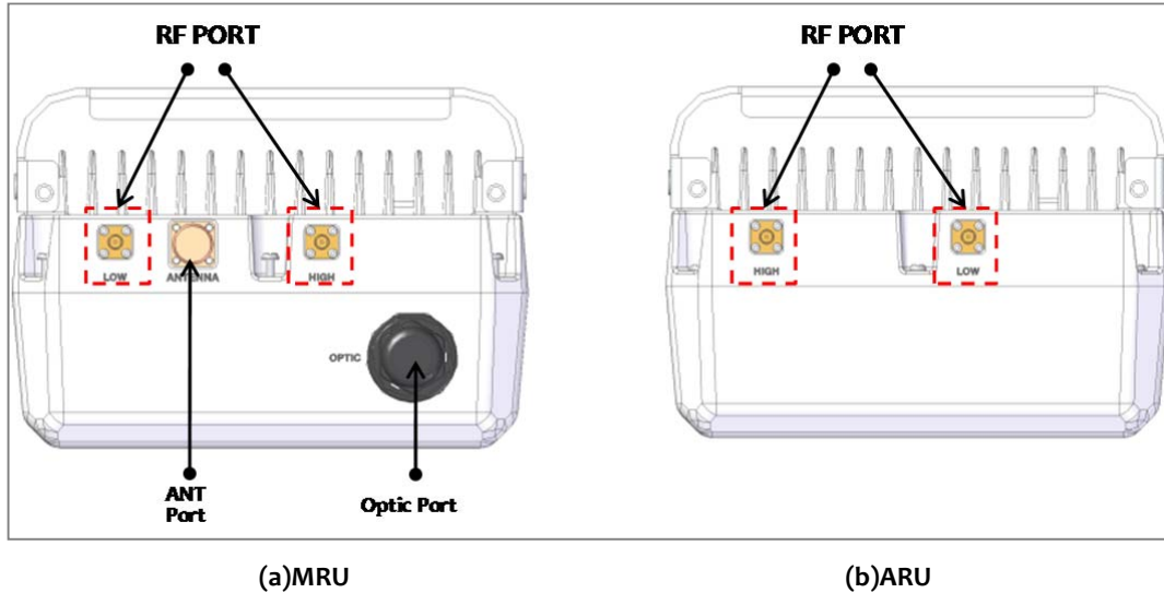
Figure 4.42 – ROU Top View for MRU 1900P+850C and ARU 700LTE+AWS-1
