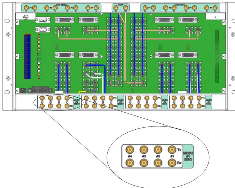
Figure 5.4 – BIU RF interface diagram
