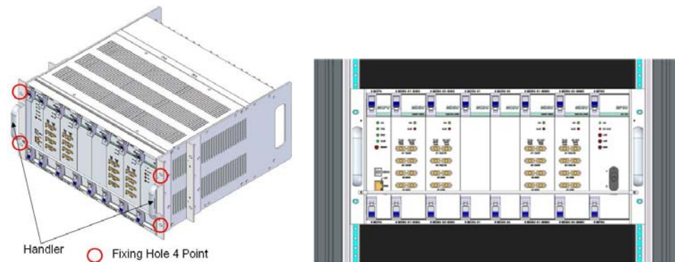
Figure 5.1 – RACK Installation
