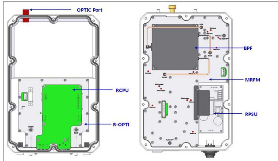
(a) MRU 1900PCS+850C
