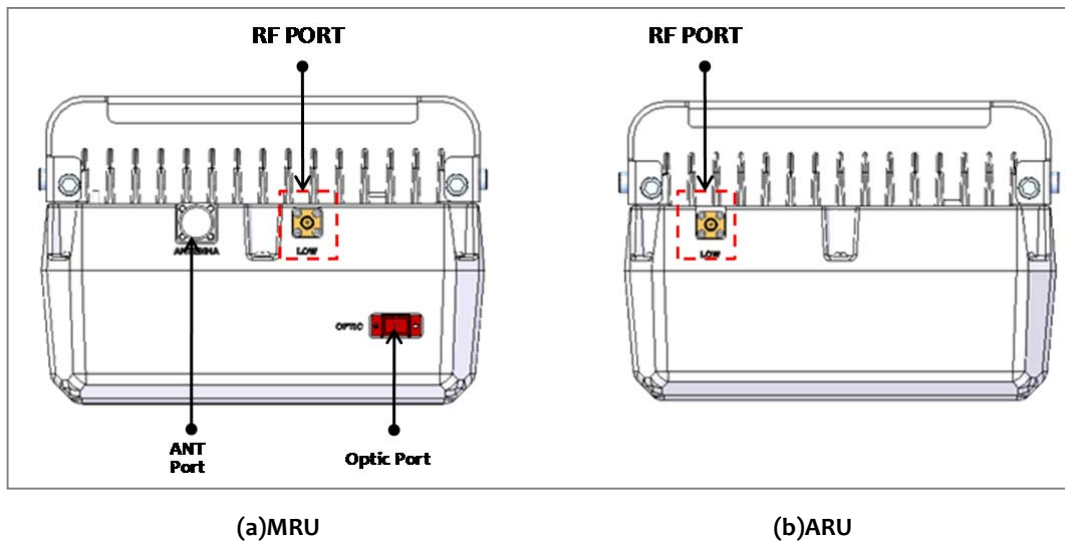
Figure 4.42 – ROU Top View for MRU 1900P and ARU 900I+800I
