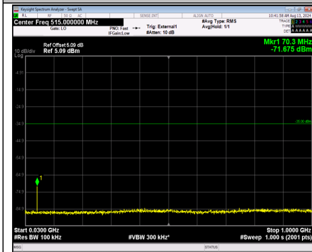
41-41-20MHz-5MHz-QPSK-QPSK-41090-41207-1RB#0-1RB#24-30~1000MHz-PASS
