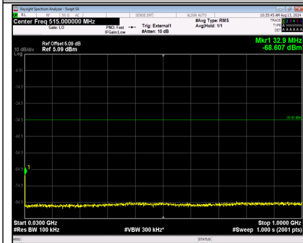
41-41-20MHz-5MHz-16QAM-16QAM-40715-40832-1RB #0-1RB#24-30~1000MHz-PASS
