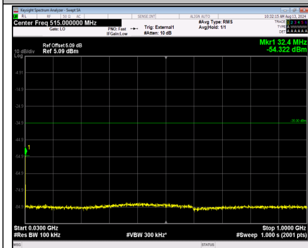
41-41-20MHz-5MHz-16QAM-16QAM-40715-40832-1RB #0-0RB#0-30~1000MHz-PASS
