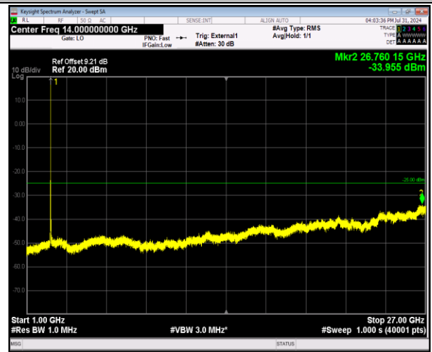
41-41-20MHz-5MHz-64QAM-64QAM-40340-40457-1RB# 99-0RB#0-1000~27000MHz-PASS
