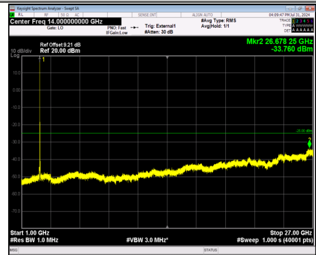
41-41-20MHz-5MHz-64QAM-64QAM-41090-41207-1RB#0-ORB#0-1000~27000MHz-PASS
