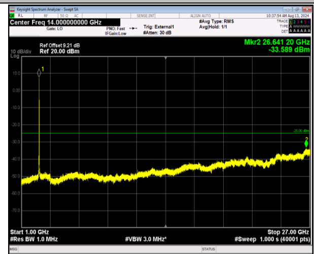
41-41-20MHz-5MHz-16QAM-16QAM-40715-40832-100R B#0-25RB#0-1000~27000MHz-PASS
