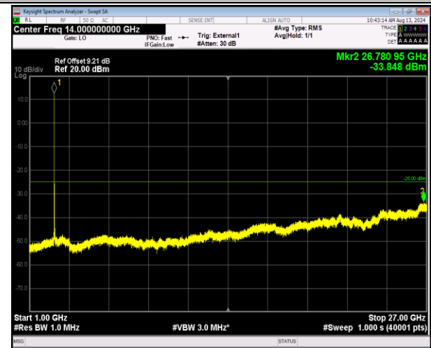
41-41-20MHz-5MHz-16QAM-16QAM-41090-41207-1RB# 0-1RB#24-1000~27000MHz-PASS
