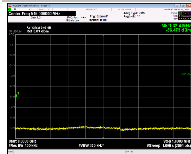
41-41-20MHz-5MHz-64QAM-64QAM-40715-40832-1RB #0-0RB#0-30~1000MHz-PASS
