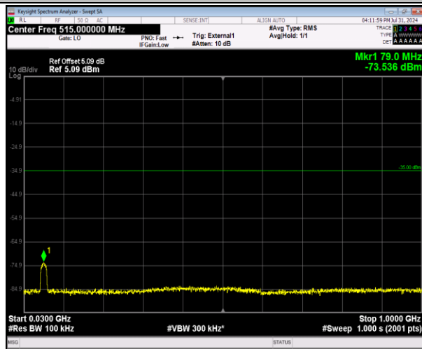
41-41-20MHz-5MHz-64QAM-64QAM-41090-41207-100 RB#0-25RB#0-30~1000MHz-PASS
