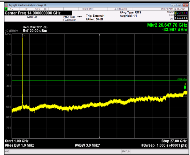
41-41-20MHz-5MHz-64QAM-64QAM-40715-40832-1RB# 99-0RB#0-1000~27000MHz-PASS
