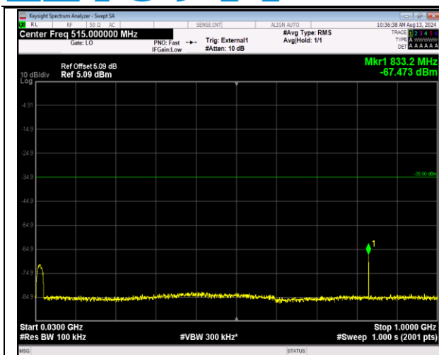
41-41-20MHz-5MHz-QPSK-QPSK-40715-40832-100RB #0-25RB#0-30~1000MHz-PASS
