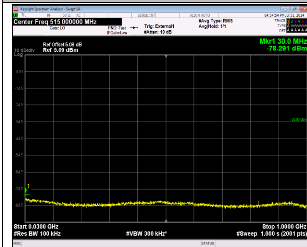
41-41-20MHz-20MHz-64QAM-64QAM-40340-40538-100 RB#0-100RB#0-30~1000MHz-PASS
