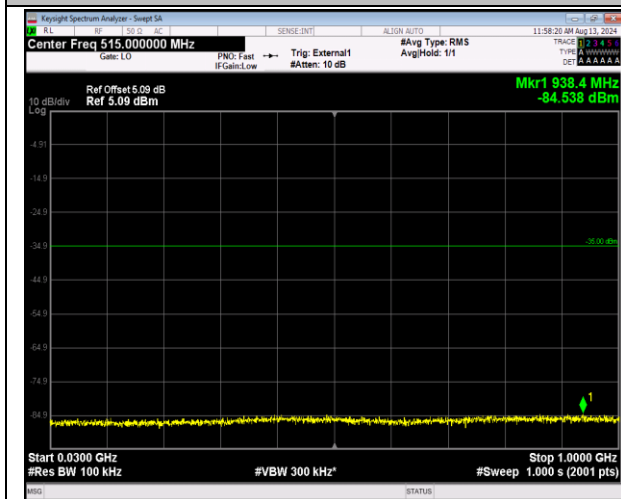
41-41-20MHz-20MHz-16QAM-16QAM-40340-40538-1R B#0-1RB#99-30~1000MHz-PASS
