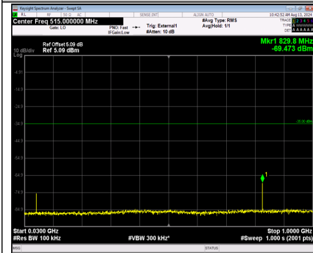
41-41-20MHz-5MHz-16QAM-16QAM-41090-41207-1RB #0-1RB#24-30~1000MHz-PASS
