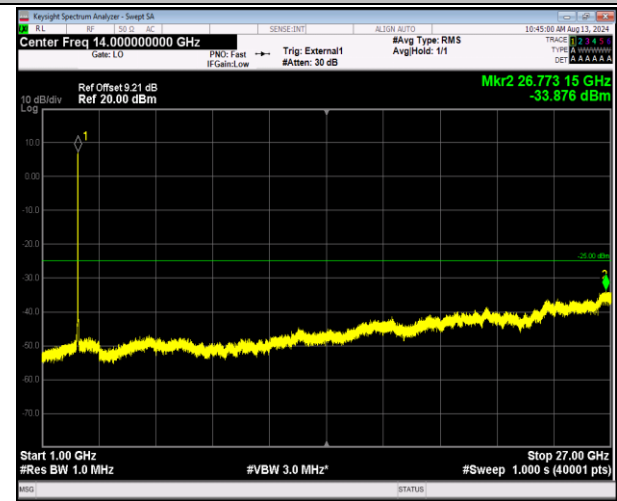
41-41-20MHz-5MHz-16QAM-16QAM-41090-41207-100RB#0-25RB#0-1000~27000MHz-PASS
