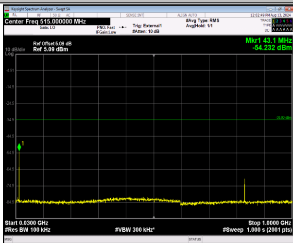
41-41-20MHz-20MHz-QPSK-QPSK-40641-40839-1RB# 99-ORB#0-30~1000MHz-PASS
