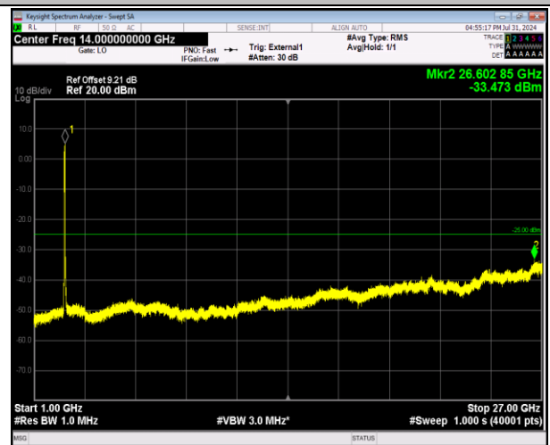
41-41-20MHz-20MHz-64QAM-64QAM-40340-40538-100 RB#0-100RB#0-1000~27000MHz-PASS
