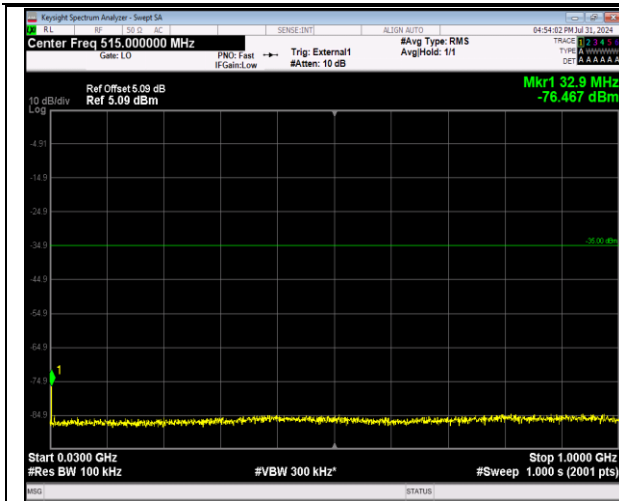
41-41-20MHz-20MHz-64QAM-64QAM-40340-40538-1R B#0-1RB#99-30~1000MHz-PASS
