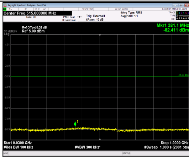
41-41-20MHz-5MHz-64QAM-64QAM-40340-40457-1RB #99-0RB#0-30~1000MHz-PASS
