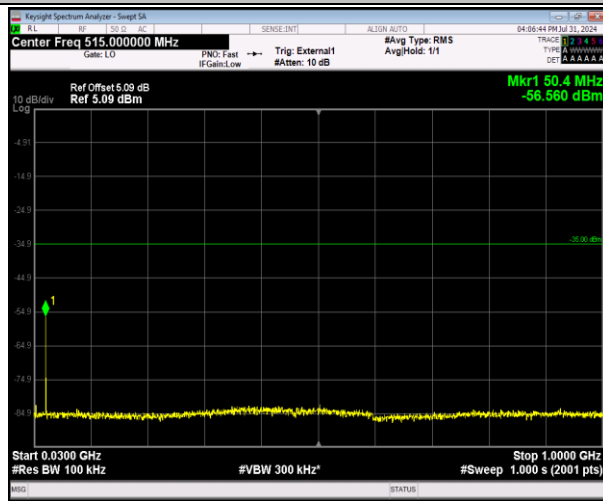
41-41-20MHz-5MHz-64QAM-64QAM-40715-40832-1RB #99-0RB#0-30~1000MHz-PASS
