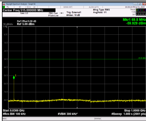
41-41-20MHz-5MHz-64QAM-64QAM-41090-41207-1RB#0-ORB#0-30~1000MHz-PASS
