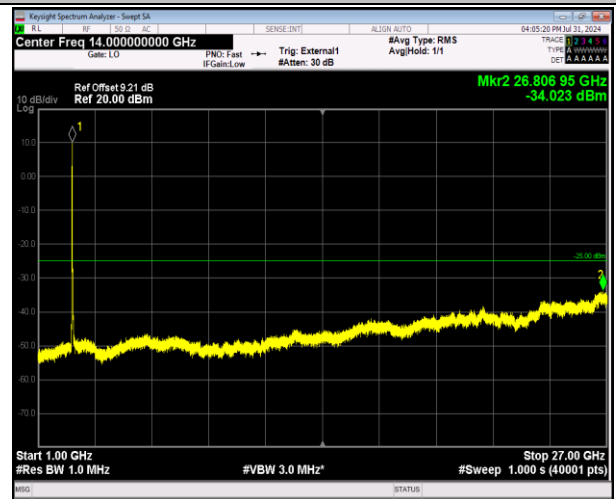
41-41-20MHz-5MHz-64QAM-64QAM-40340-40457-100R B#0-25RB#0-1000~27000MHz-PASS
