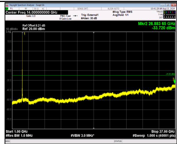
41-41-20MHz-5MHz-16QAM-16QAM-41090-41207-1RB# 99-ORB#0-1000~27000MHz-PASS
