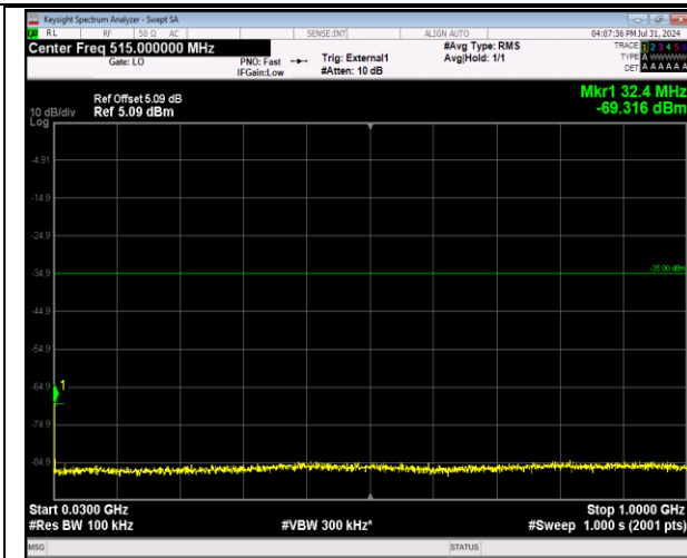
41-41-20MHz-5MHz-64QAM-64QAM-40715-40832-1RB #0-1RB#24-30~1000MHz-PASS
