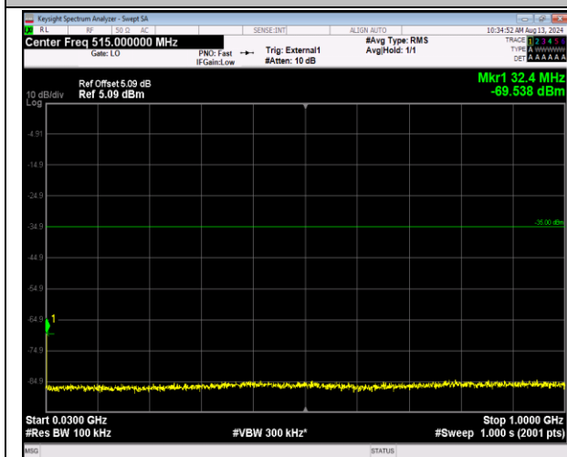
41-41-20MHz-5MHz-QPSK-QPSK-40715-40832-1RB#0-1RB#24-30~1000MHz-PASS
