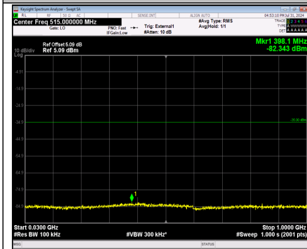
41-41-20MHz-20MHz-64QAM-64QAM-40340-40538-1R B#99-0RB#0-30~1000MHz-PASS
