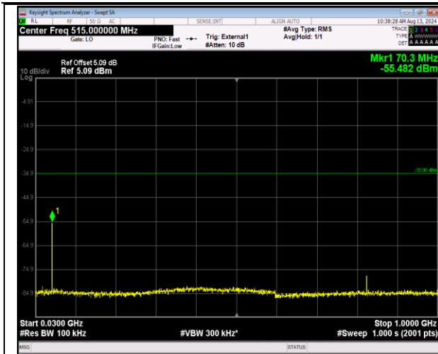
41-41-20MHz-5MHz-QPSK-QPSK-41090-41207-1RB#0-ORB#0-30~1000MHz-PASS
