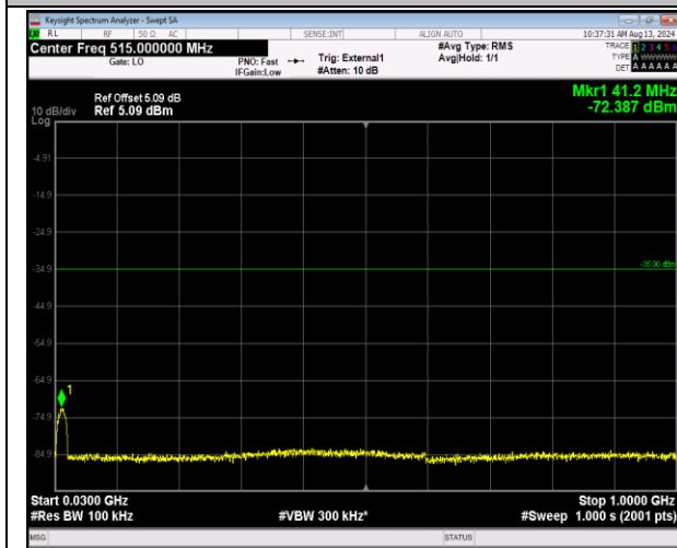
41-41-20MHz-5MHz-16QAM-16QAM-40715-40832-100 RB#0-25RB#0-30~1000MHz-PASS
