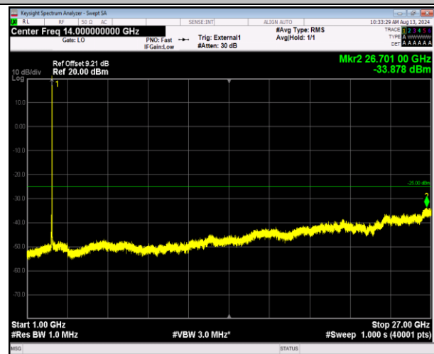
41-41-20MHz-5MHz-QPSK-QPSK-40715-40832-1RB#99-ORB#0-1000~27000MHz-PASS
