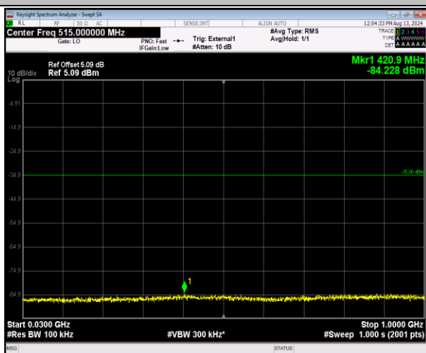
41-41-20MHz-20MHz-QPSK-QPSK-40641-40839-1RB# 0-1RB#99-30~1000MHz-PASS
