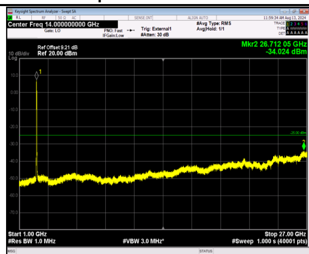
41-41-20MHz-20MHz-QPSK-QPSK-40340-40538-100RB #0-100RB#0-1000~27000MHz-PASS
