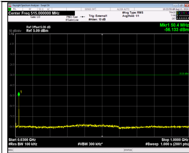
41-41-20MHz-5MHz-16QAM-16QAM-40715-40832-1RB #99-ORB#0-30~1000MHz-PASS
