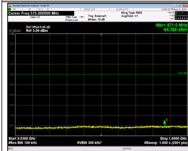
41-41-20MHz-20MHz-16QAM-16QAM-40641-40839-1R B#0-1RB#99-30~1000MHz-PASS
