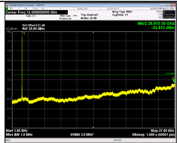
41-41-20MHz-5MHz-16QAM-16QAM-40715-40832-1RB# 99-ORB#0-1000~27000MHz-PASS
