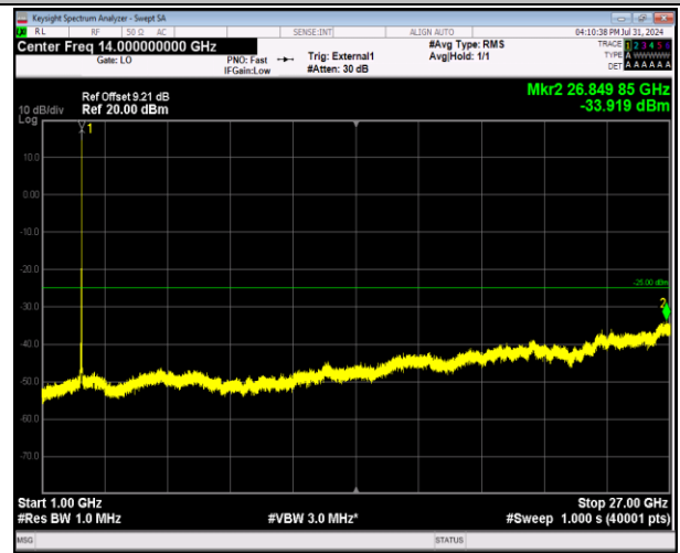
41-41-20MHz-5MHz-64QAM-64QAM-41090-41207-1RB# 99-0RB#0-1000~27000MHz-PASS
