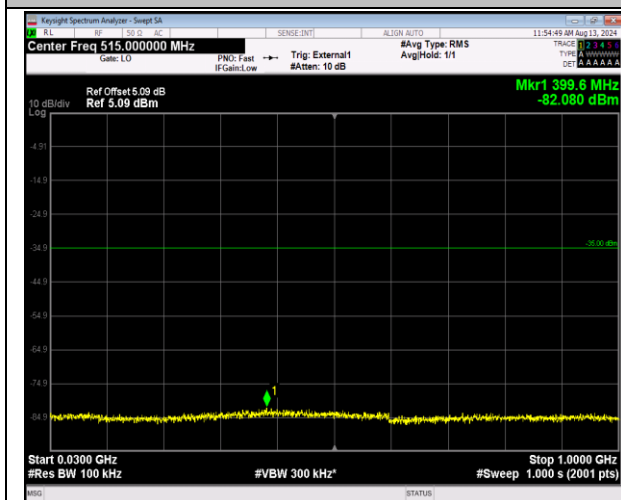
41-41-20MHz-20MHz-16QAM-16QAM-40340-40538-1R B#0-0RB#0-30~1000MHz-PASS
