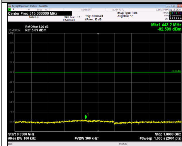
41-41-20MHz-20MHz-16QAM-16QAM-40641-40839-1R B#0-0RB#0-30~1000MHz-PASS
