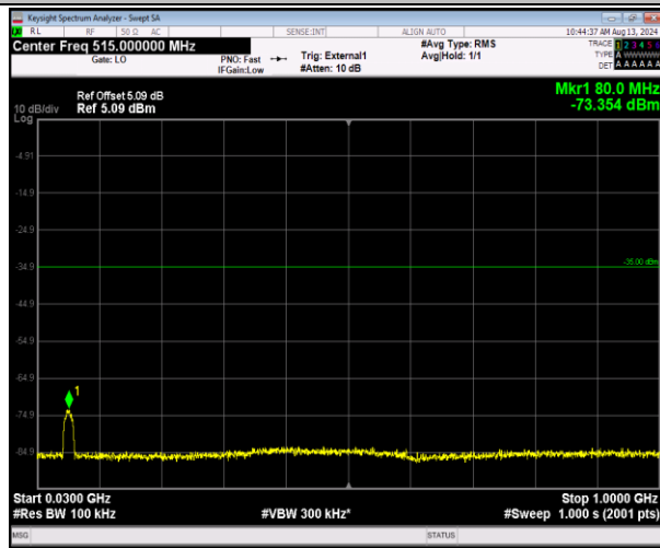
41-41-20MHz-5MHz-16QAM-16QAM-41090-41207-100RB#0-25RB#0-30~1000MHz-PASS
