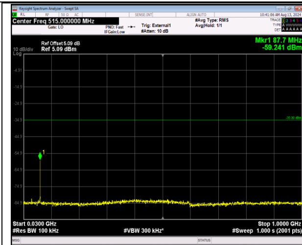
41-41-20MHz-5MHz-16QAM-16QAM-41090-41207-1RB #99-ORB#0-30~1000MHz-PASS
