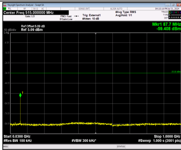
41-41-20MHz-5MHz-64QAM-64QAM-41090-41207-1RB #99-0RB#0-30~1000MHz-PASS
