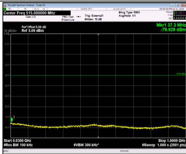
41-41-20MHz-5MHz-64QAM-64QAM-40340-40457-100 RB#0-25RB#0-30~1000MHz-PASS
