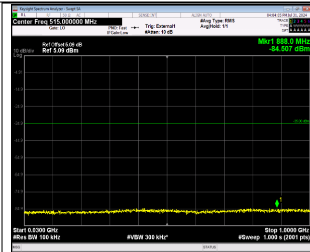
41-41-20MHz-5MHz-64QAM-64QAM-40340-40457-1RB #0-1RB#24-30~1000MHz-PASS
