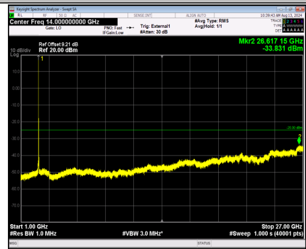
41-41-20MHz-5MHz-16QAM-16QAM-41090-41207-1RB# 0-0RB#0-1000~27000MHz-PASS
