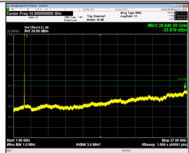
41-41-20MHz-5MHz-QPSK-QPSK-41090-41207-1RB#99-ORB#0-1000~27000MHz-PASS
