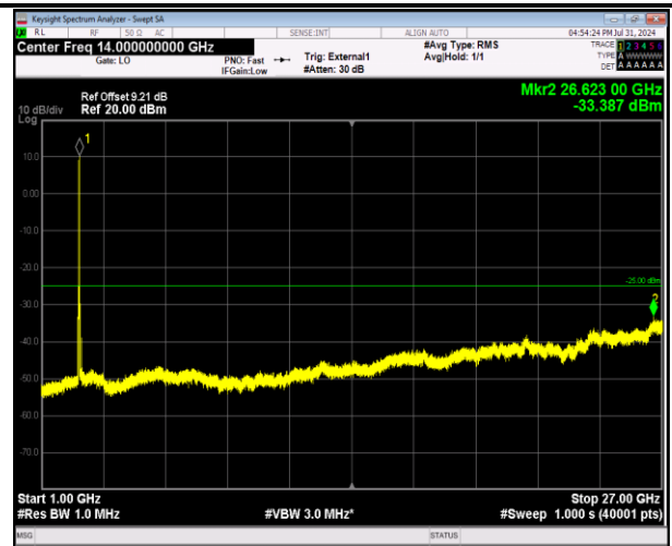
41-41-20MHz-20MHz-64QAM-64QAM-40340-40538-1RB #0-1RB#99-1000~27000MHz-PASS
