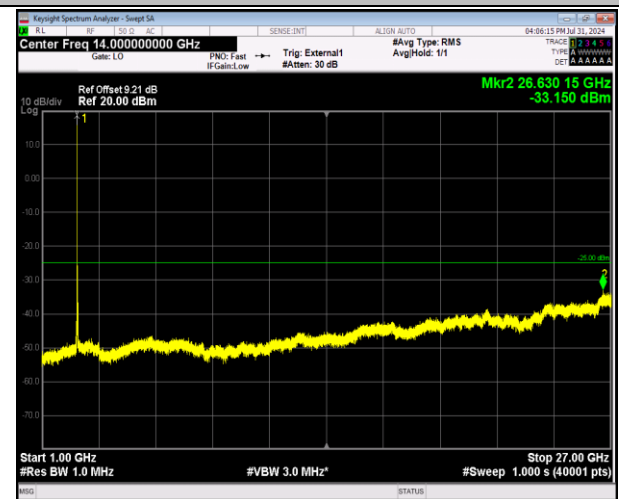
41-41-20MHz-5MHz-64QAM-64QAM-40715-40832-1RB# 0-0RB#0-1000~27000MHz-PASS
