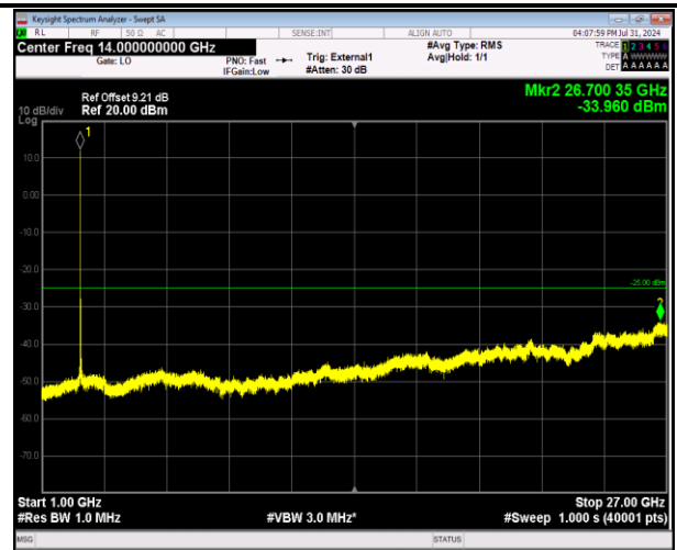
41-41-20MHz-5MHz-64QAM-64QAM-40715-40832-1RB# 0-1RB#24-1000~27000MHz-PASS
