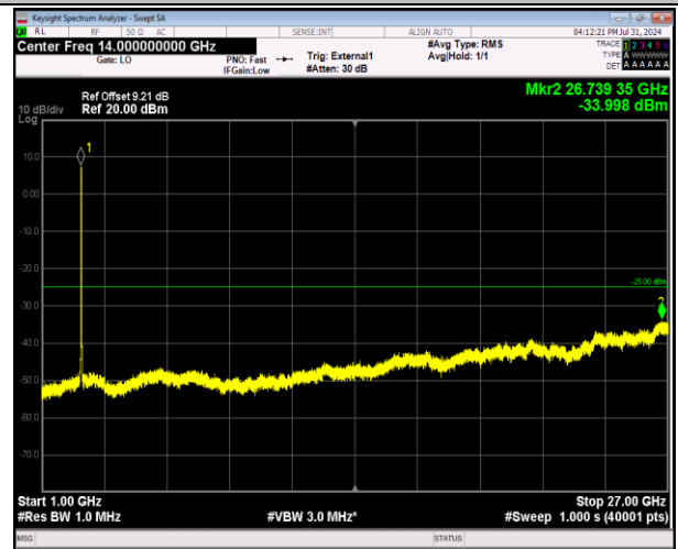
41-41-20MHz-5MHz-64QAM-64QAM-41090-41207-100R B#0-25RB#0-1000~27000MHz-PASS
