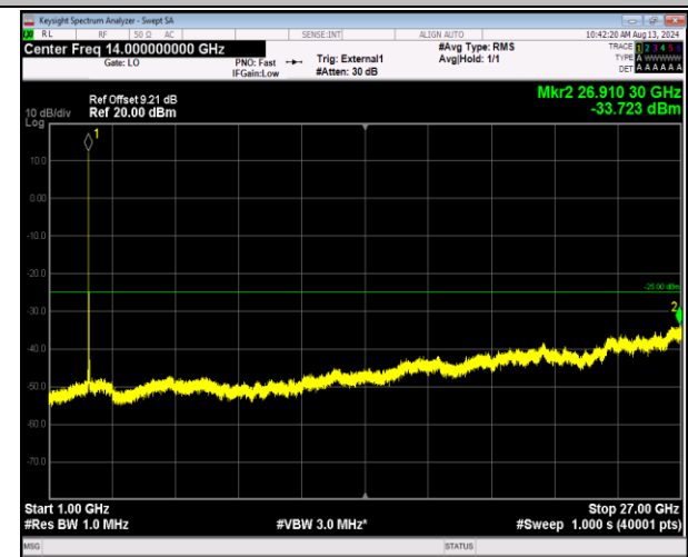
41-41-20MHz-5MHz-QPSK-QPSK-41090-41207-1RB#0-1RB#24-1000~27000MHz-PASS
