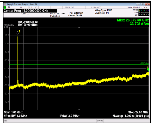
41-41-20MHz-5MHz-64QAM-64QAM-40340-40457-1RB# 0-1RB#24-1000~27000MHz-PASS
