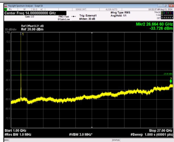
41-41-20MHz-5MHz-16QAM-16QAM-40715-40832-1RB# 0-0RB#0-1000~27000MHz-PASS
