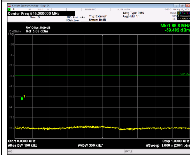
41-41-20MHz-5MHz-16QAM-16QAM-41090-41207-1RB #0-0RB#0-30~1000MHz-PASS
