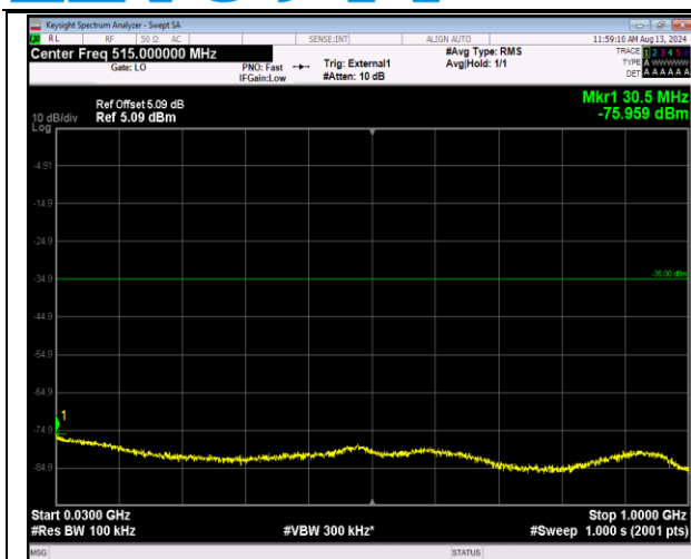
41-41-20MHz-20MHz-QPSK-QPSK-40340-40538-100R B#0-100RB#0-30~1000MHz-PASS
