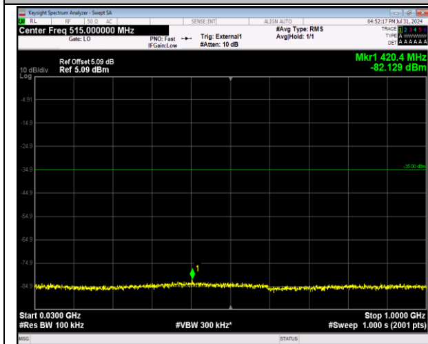
41-41-20MHz-20MHz-64QAM-64QAM-40340-40538-1R B#0-ORB#0-30~1000MHz-PASS
