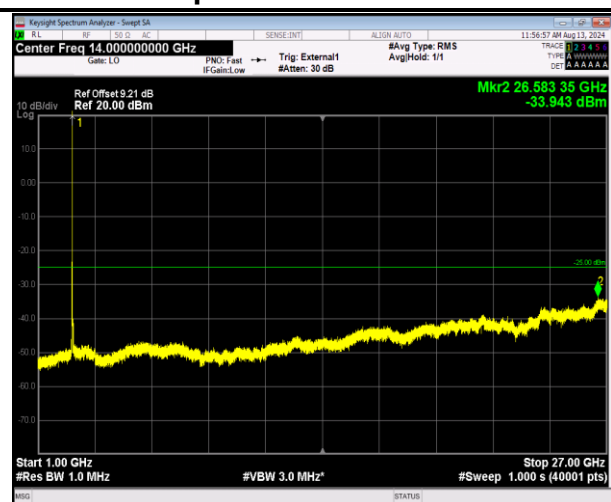
41-41-20MHz-20MHz-16QAM-16QAM-40340-40538-1RB #99-ORB#0-1000~27000MHz-PASS
