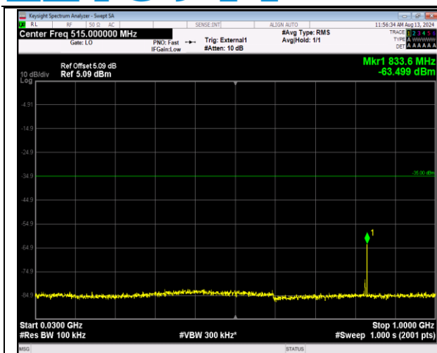
41-41-20MHz-20MHz-16QAM-16QAM-40340-40538-1R B#99-ORB#0-30~1000MHz-PASS
