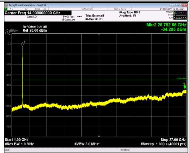
41-41-20MHz-5MHz-64QAM-64QAM-40715-40832-100R B#0-25RB#0-1000~27000MHz-PASS
