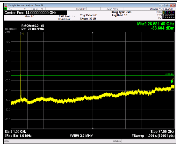
41-41-20MHz-20MHz-64QAM-64QAM-40340-40538-1RB #99-0RB#0-1000~27000MHz-PASS
