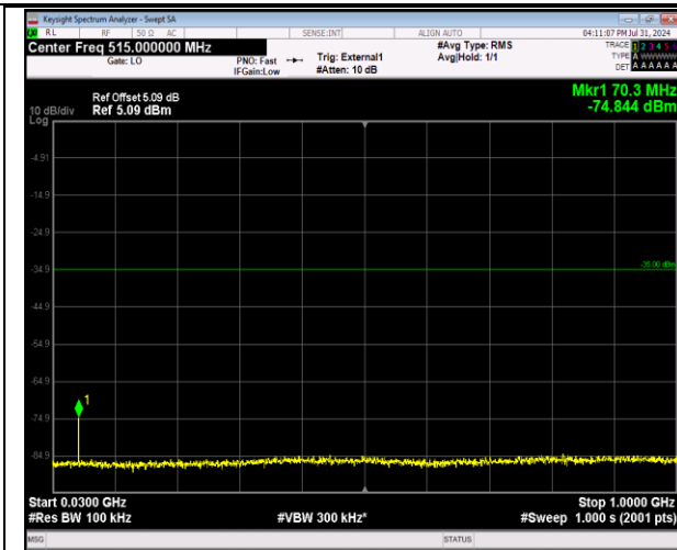
41-41-20MHz-5MHz-64QAM-64QAM-41090-41207-1RB #0-1RB#24-30~1000MHz-PASS
