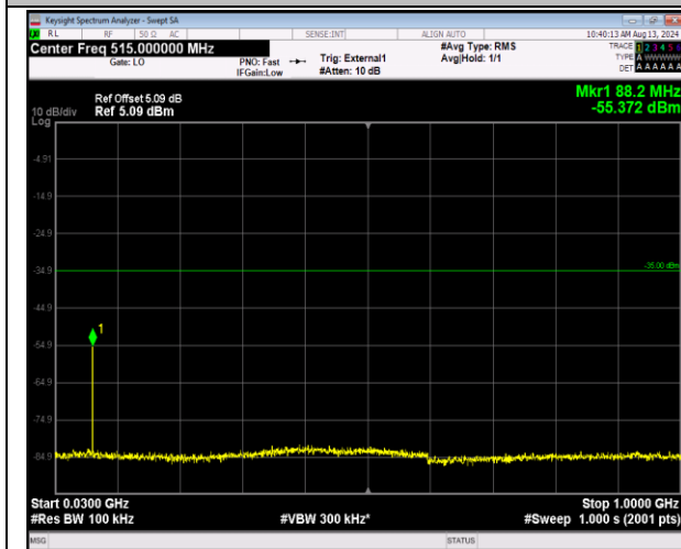
41-41-20MHz-5MHz-QPSK-QPSK-41090-41207-1RB#9-0RB#0-30~1000MHz-PASS
