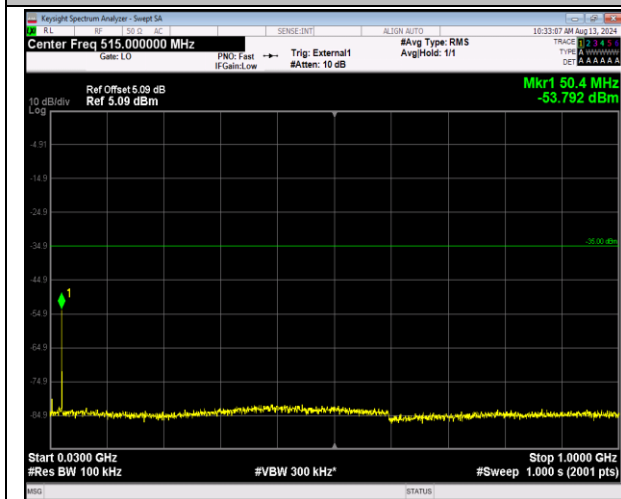
41-41-20MHz-5MHz-QPSK-QPSK-40715-40832-1RB#9-0RB#0-30~1000MHz-PASS
