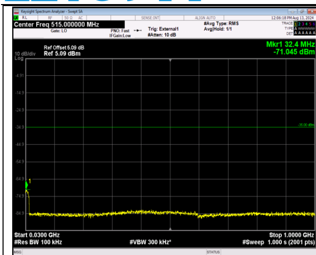
41-41-20MHz-20MHz-QPSK-QPSK-40641-40839-100R B#0-100RB#0-30~1000MHz-PASS
