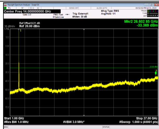
41-41-20MHz-20MHz-64QAM-64QAM-40340-40538-1RB #0-ORB#0-1000~27000MHz-PASS
