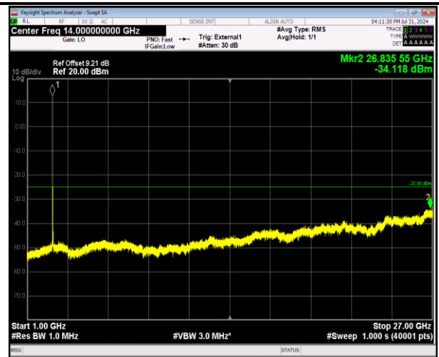
41-41-20MHz-5MHz-64QAM-64QAM-41090-41207-1RB# 0-1RB#24-1000~27000MHz-PASS
