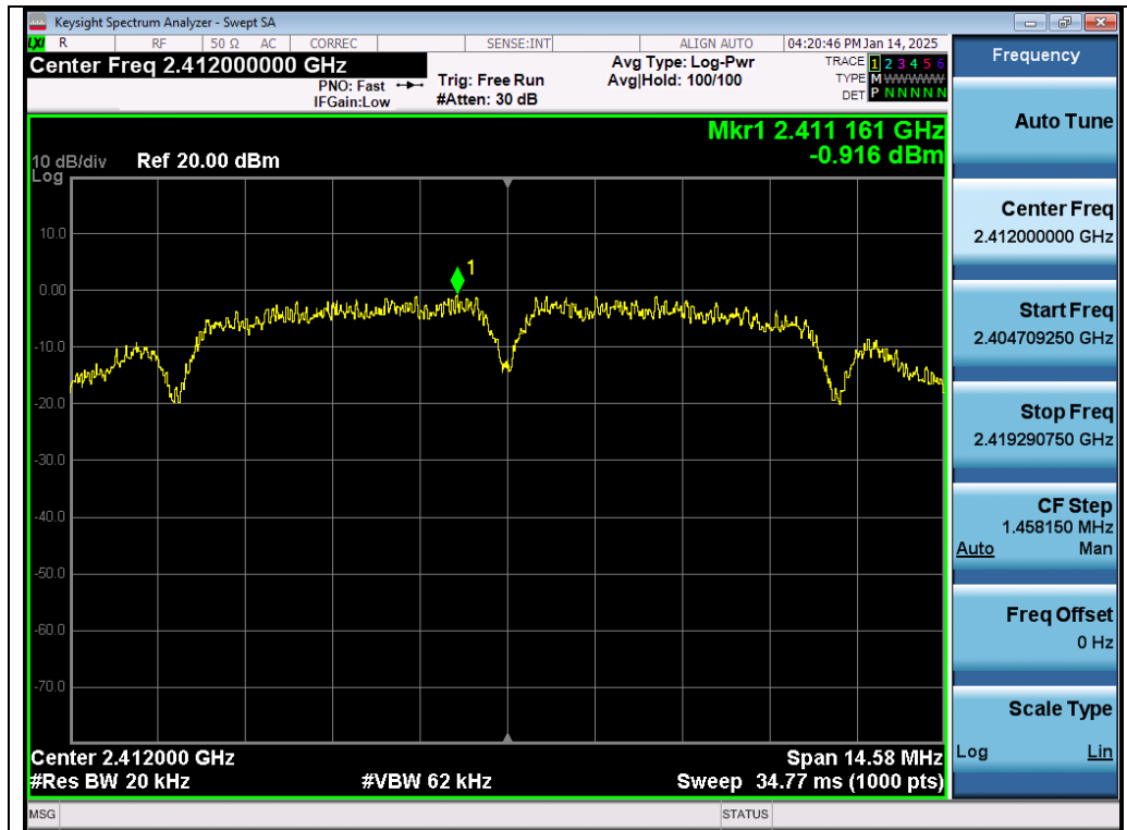
Test_Graph_802.11b_Chain A_2412_1Mbps_PSD
