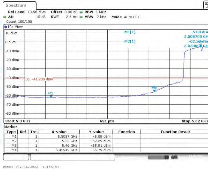
11N40SISO_Ant1_Low_5510_Peak
