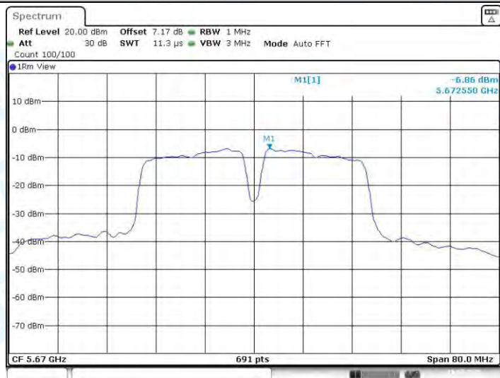
11AC40SISO_Ant1_5670
