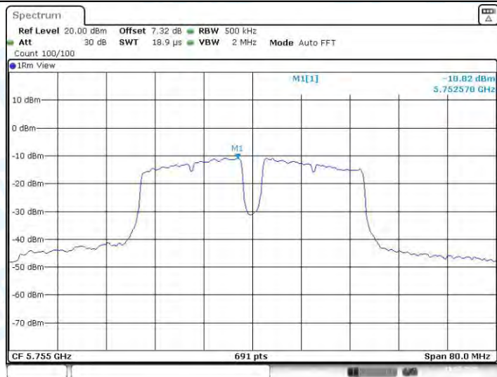
11AC40SISO_Ant1_5755
