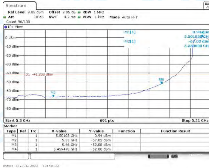
11A_Ant1_Low_5500_Peak
