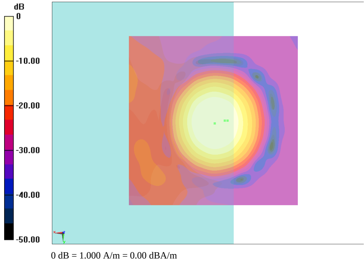
Fig B.6 T-Coil GSM 1900
