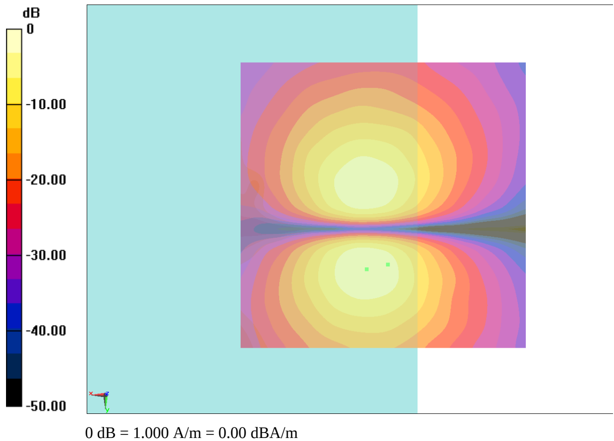
Fig B.5 T-Coil GSM 1900
