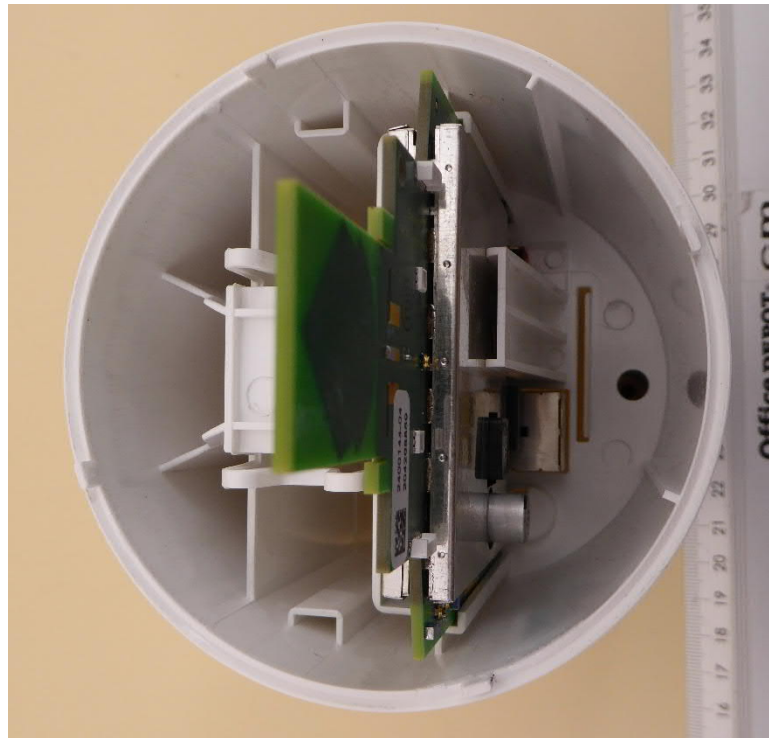
Internal view 2
