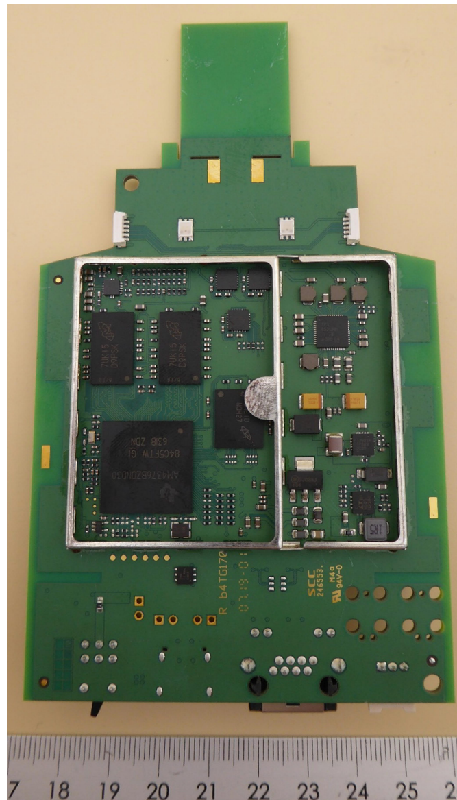
PCB, bottom view (shielding removed)
