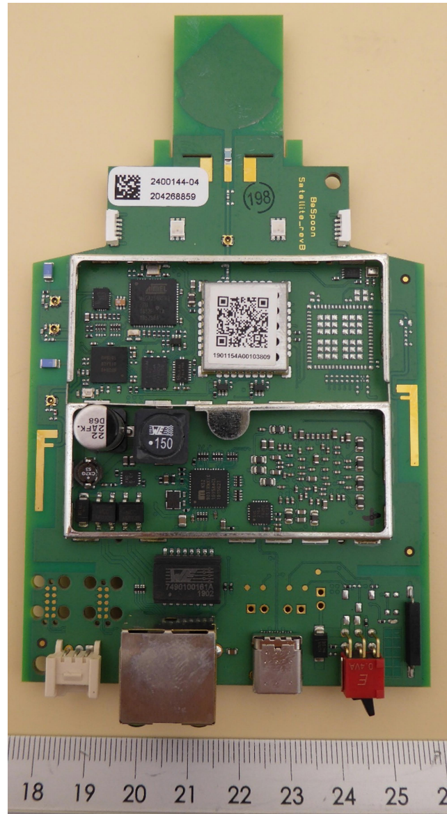
PCB, top view (shielding removed)
