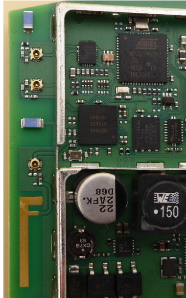
IEEE 802.15.4 radio part (detail view)
