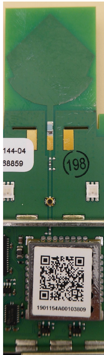
UWB radio part (detail view)
