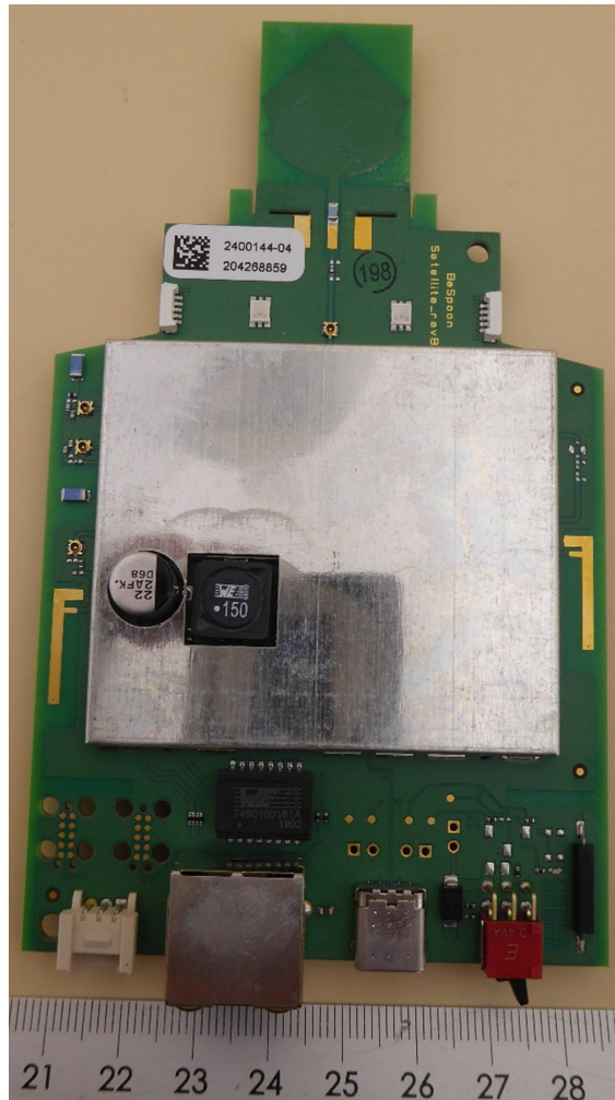
PCB, top view
