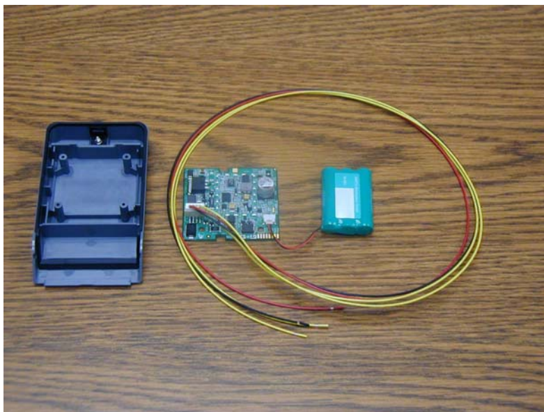
Original VAM module disassembled showing housing, PCBA, cable, and backup battery.
